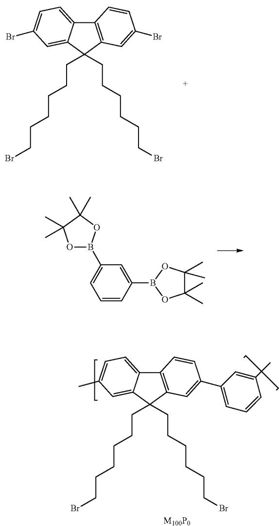
Scheme 2: Synthesis of a conjugated polymer
