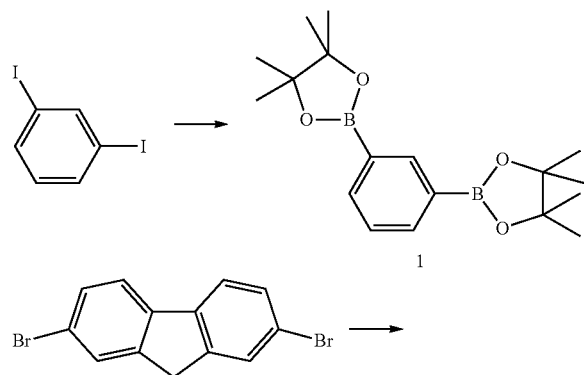
Scheme 1: Synthesis of an aromatic repeat unit
