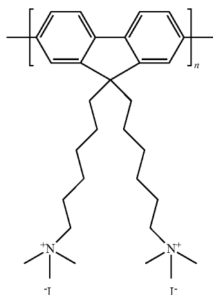
polymer 1
