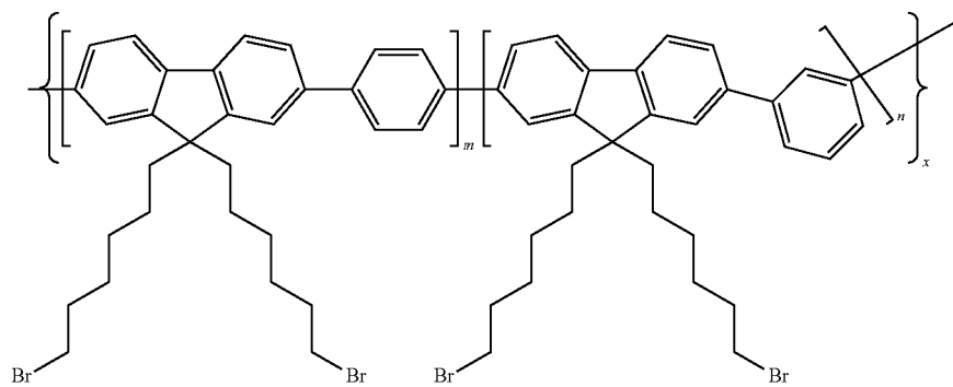
Scheme 4: Derivatization of a conjugated polymer
