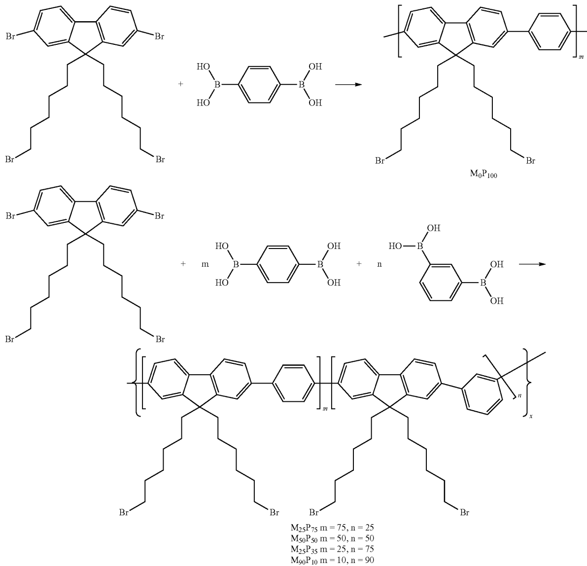
Scheme 3: Synthesis of a conjugated polymer
