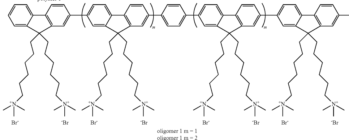
polymer 1
