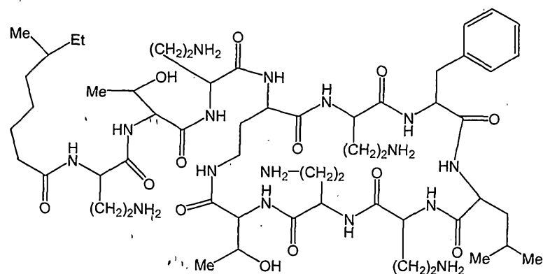
Polymyxin B
