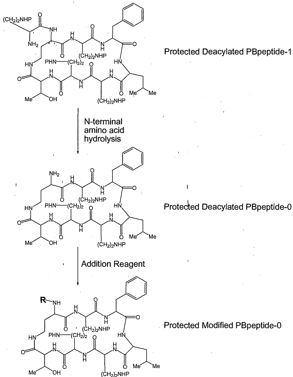
Scheme IV
