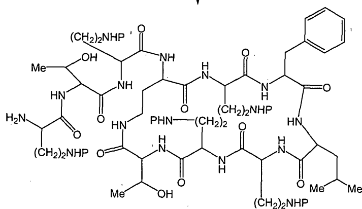
Protected Deacylated PBpeptide-3
