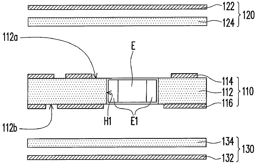
FIG. 1C(PRIOR ART)
