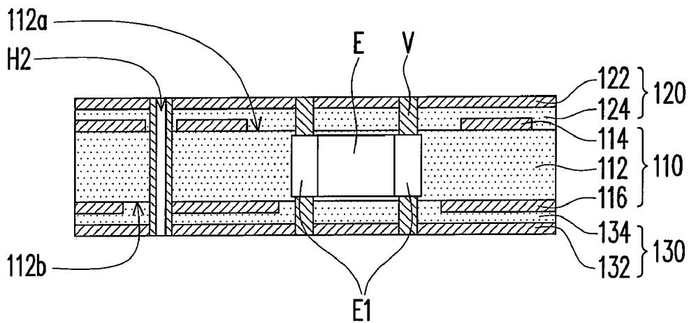
FIG. 1D(PRIOR ART)
