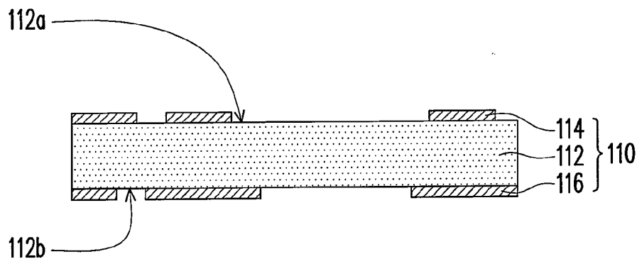
FIG. 1A(PRIOR ART)
