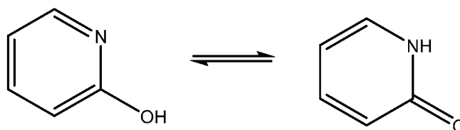
2-hydroxy pyridine
