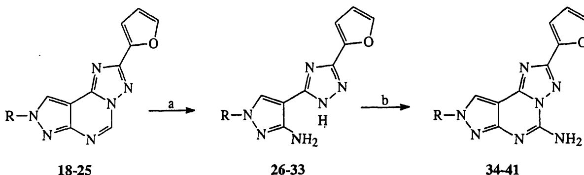
Scheme VII: General procedures for the preparation of 5-Amino-8-(ar)alkyl-2-(2-furyl)-pyrazolo[4,3-e] 1,2,4-triazolo[1,5-c]pyrimidine (33-40)
