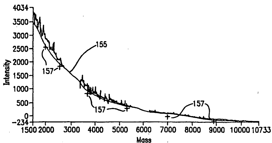
FIG. 37 FIND MINIMA IN REMAINING SIGNALS AND CONNECT TO FORM A PEAK FREE SIGNAL
