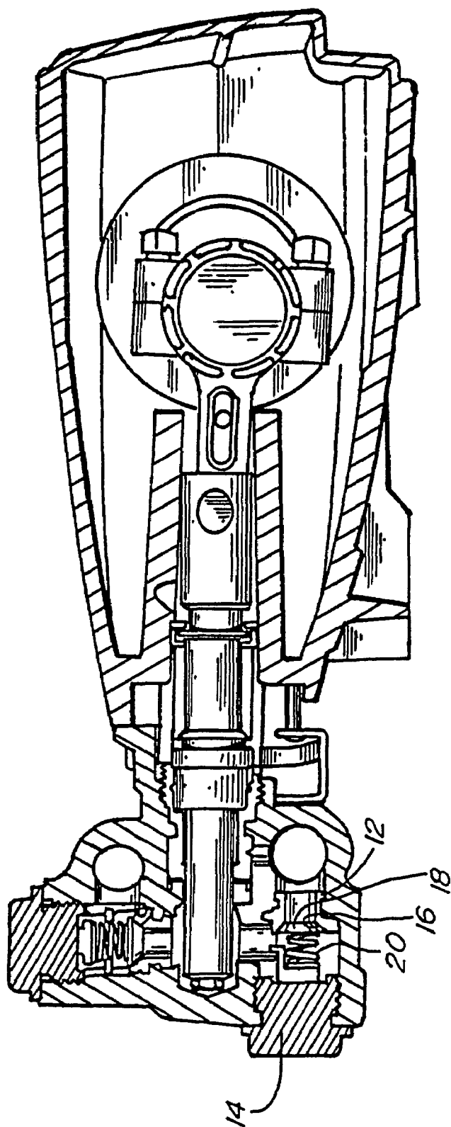
Fig. 2. PRIOR ART
