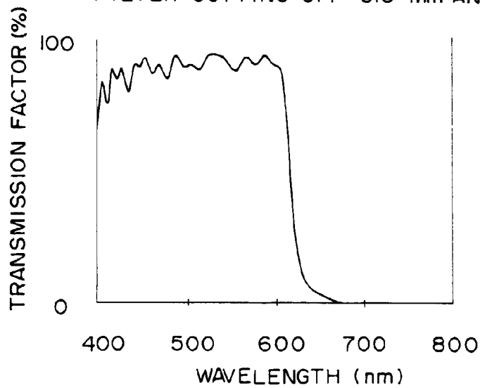
FILTER CUTTING OFF 615 nm AND LONGER
