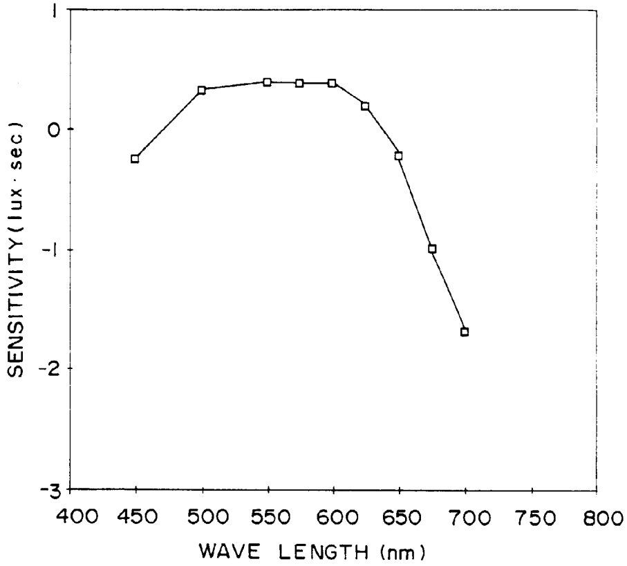
SPECTRAL SENSITIVITY CHARACTERISTICS
