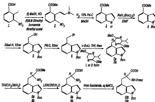
Synthesis of (DL)-Neo-Tryptophan
