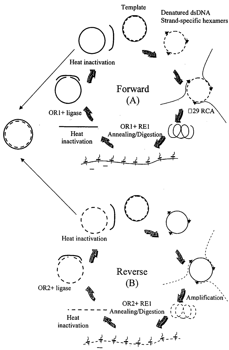
Figure 3 Amplification of Forward and Reverse DNA strands.
