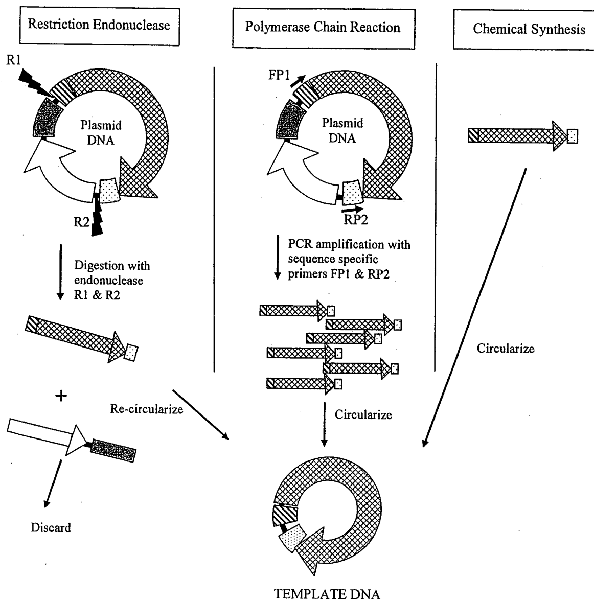
Figure 1 Template Synthesis
