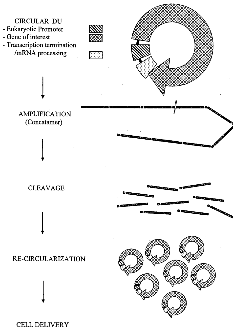
Figure 2 In Vitro Amplification Process
