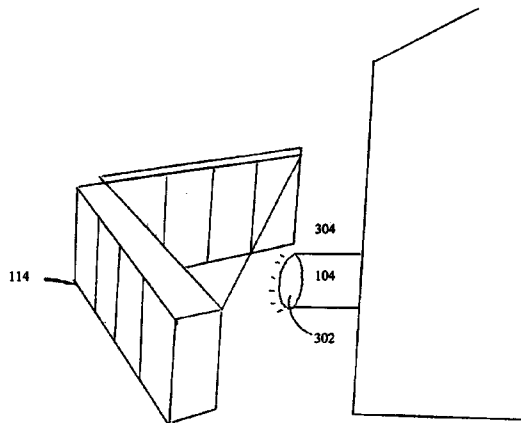
104 - Ventilation exhaust ports 114 - Side filter system 302 - Exhaust fan outlet end 304 - Alternate exhaust air escape opening
