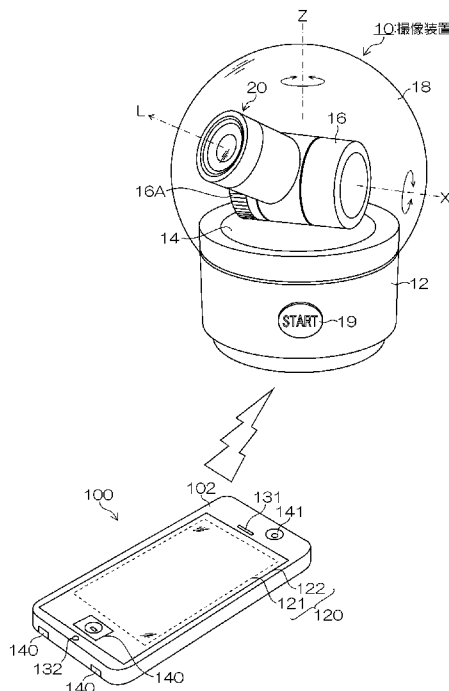
10 Imaging device
