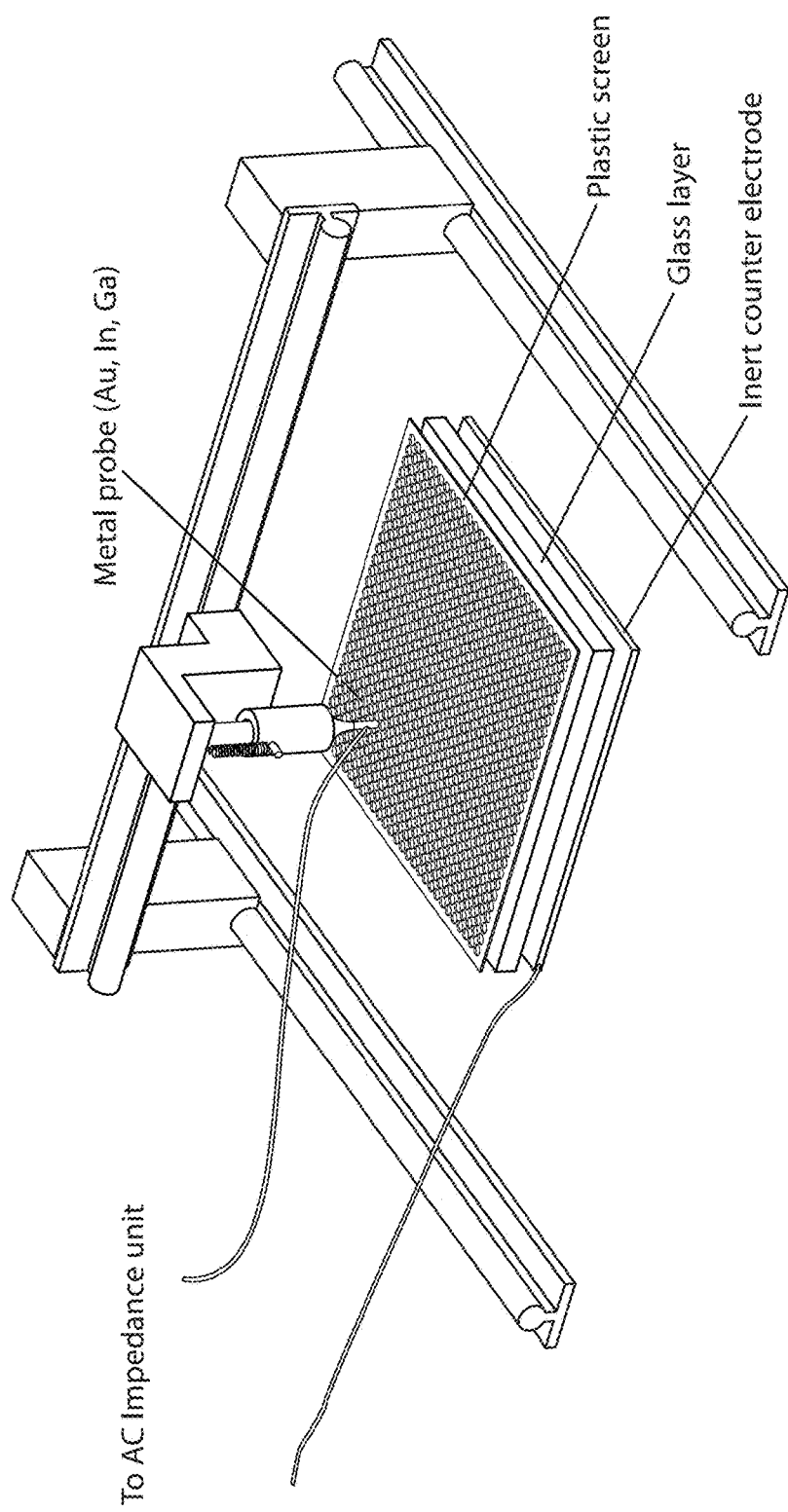
Measurements of local resistance in glass electrolyte
