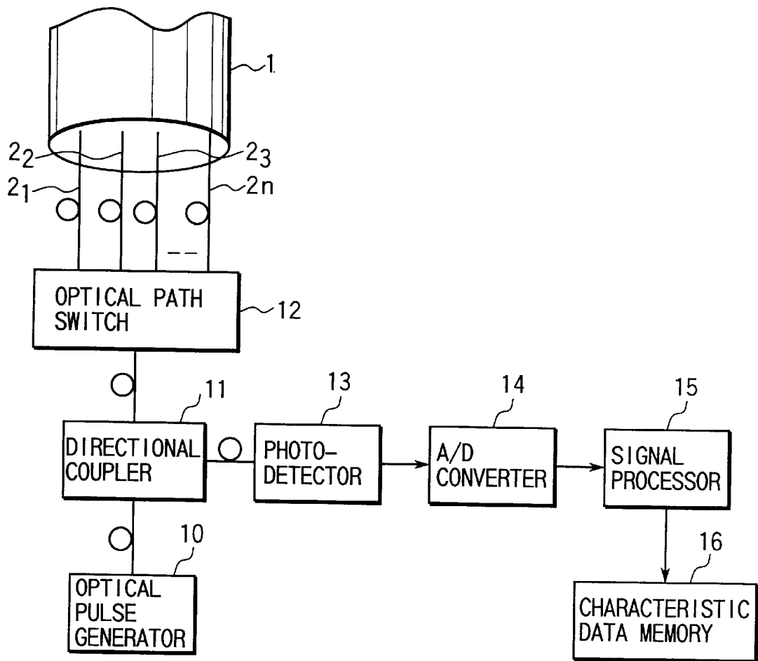
FIG. 10 (PRIOR ART)
