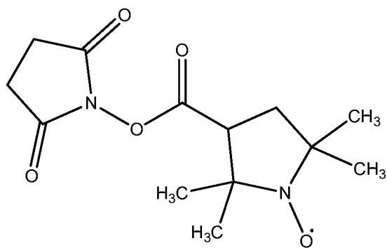
3-Succinimidyl-Carboxy-PROXYL (3-SCP; 1-(((2,2,5,5-tetramethyl-1-pyrrolidinyloxy)-3-carbonyloxy)-2,5-pyrrolidinedione).
