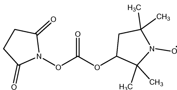
3-Succinimidyl-PROXYL-Carbonate (3-SPC; 1-(((2,2,5,5-tetramethyl-1-pyrrolidinyloxy)-3-oxycarbonyl)oxy)-2,5-pyrrolidinedione)
