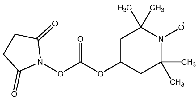
4-Succinimidyl-TEMPO-Carbonate (4-STC; 1-(((2,2,6,6-tetramethyl-1-piperidinyloxy)-4-oxycarbonyl)oxy)-2,5-pyrrolidinedione)
