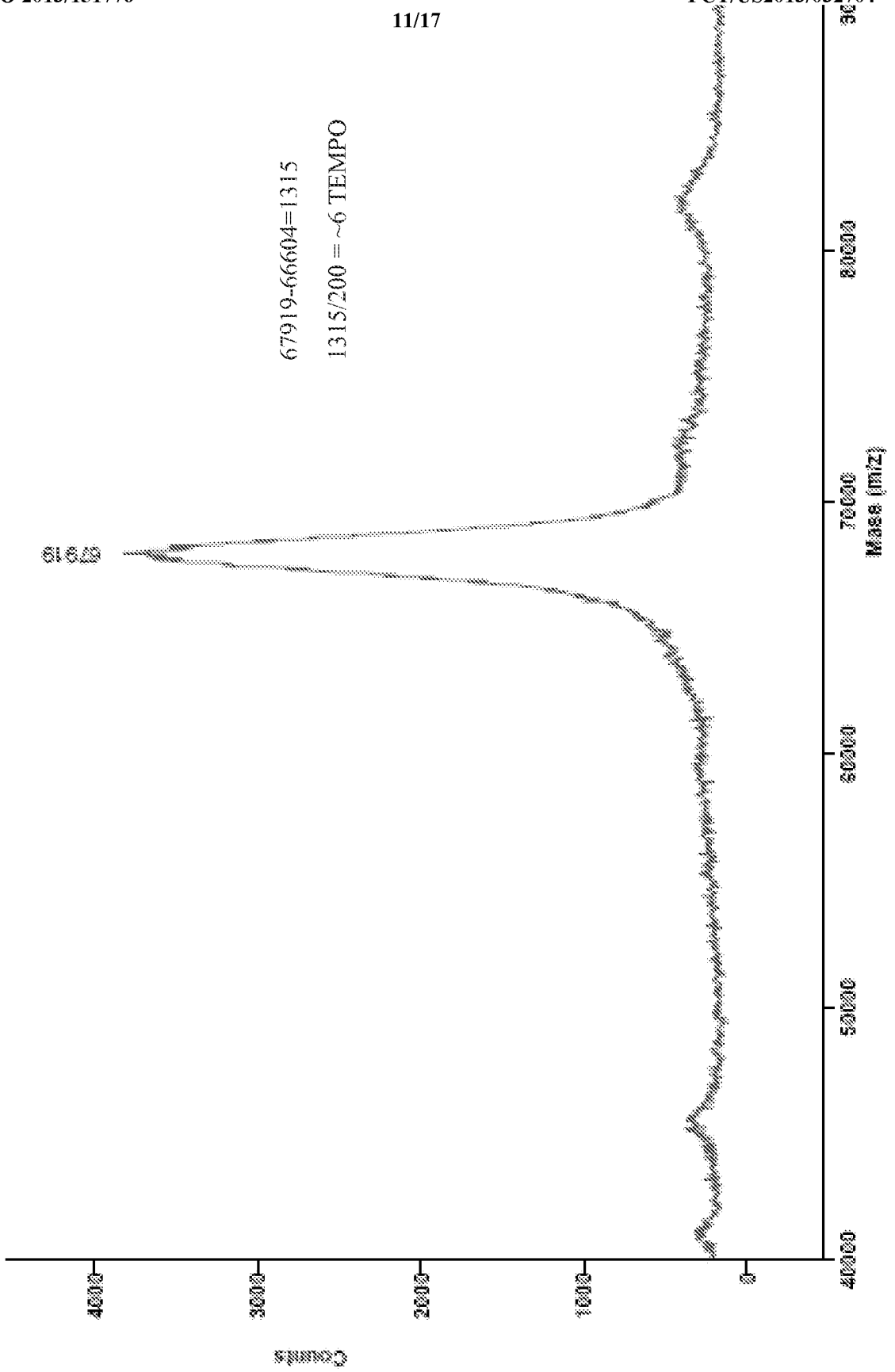
MALDI-TOF analysis of HSA + SC-TEMPO (1:10)
