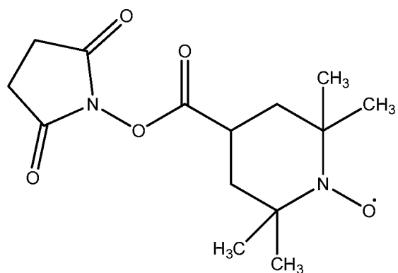
4-succinimidyl-carboxy-TEMPO (4-SCT; 1-(((2,2,6,6-tetramethyl-1-piperidinyloxy)-4-carbonyl)oxy)-2,5-pyrrolidinedione)
