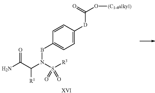
Reaction Scheme 6
