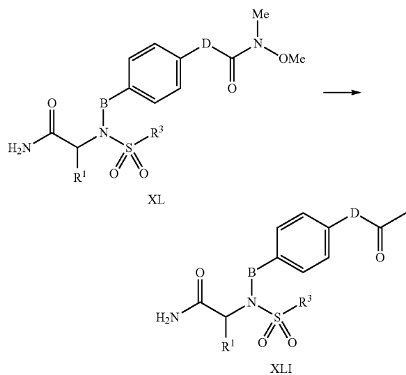
Reaction Scheme 16
