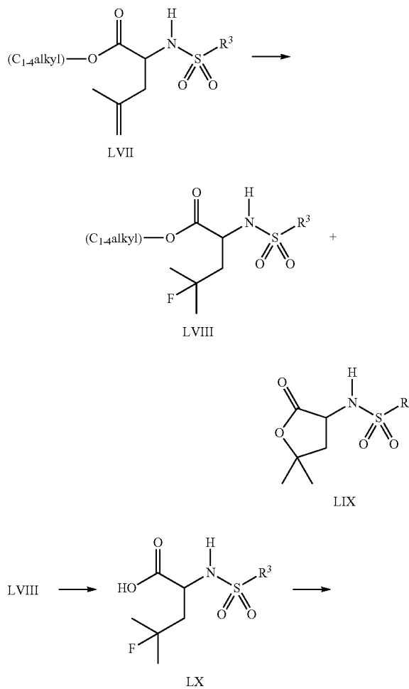
Reaction Scheme 21
