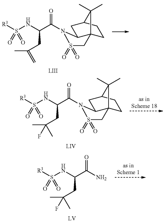
Reaction Scheme 20
