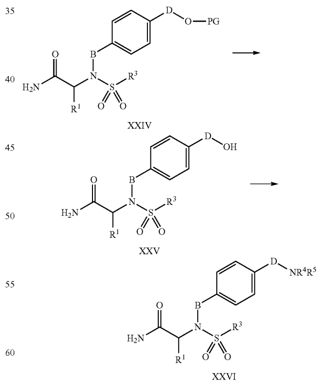
Reaction Scheme 8
