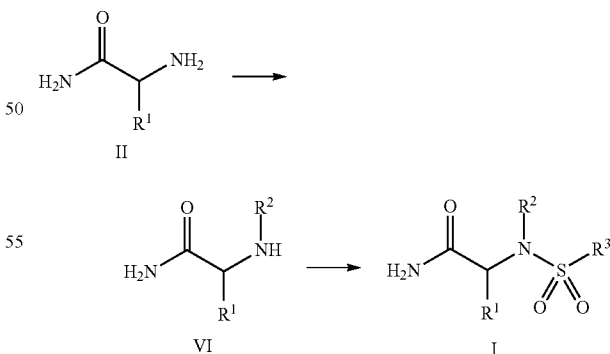
Reaction Scheme 2
