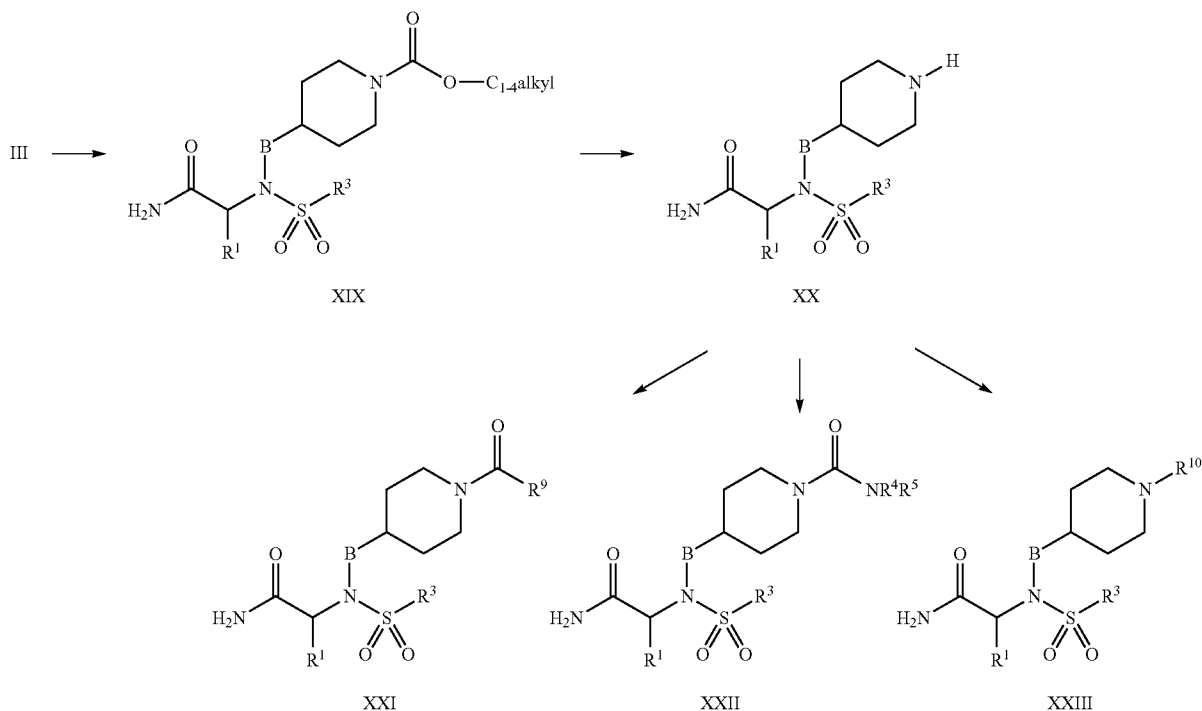
Reaction Scheme 7
