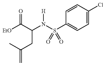
Ethyl 2-(4-chlorobenzenesulfonylamino)-4-methyl-4-pentenoate
