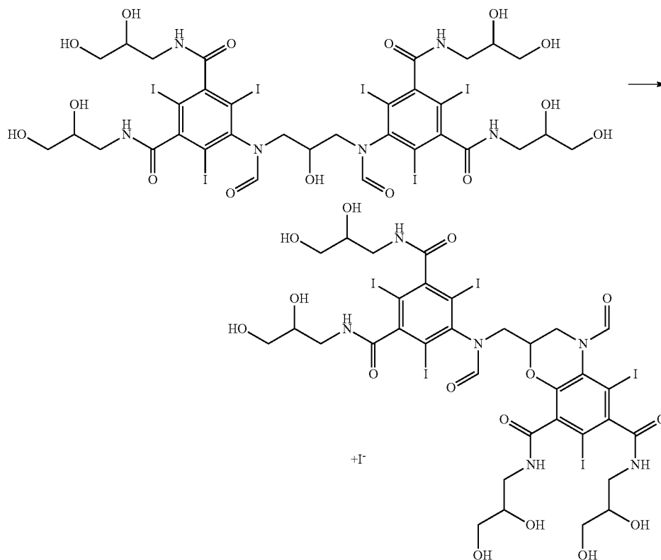
Scheme 1. Cleavage of iodide from Compound I.
