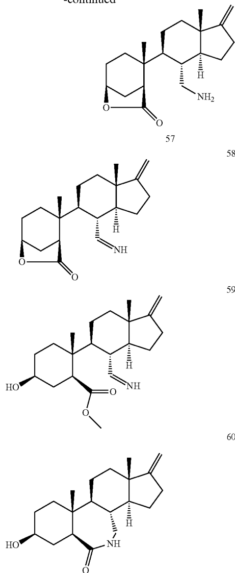
REACTION SCHEME 18:
