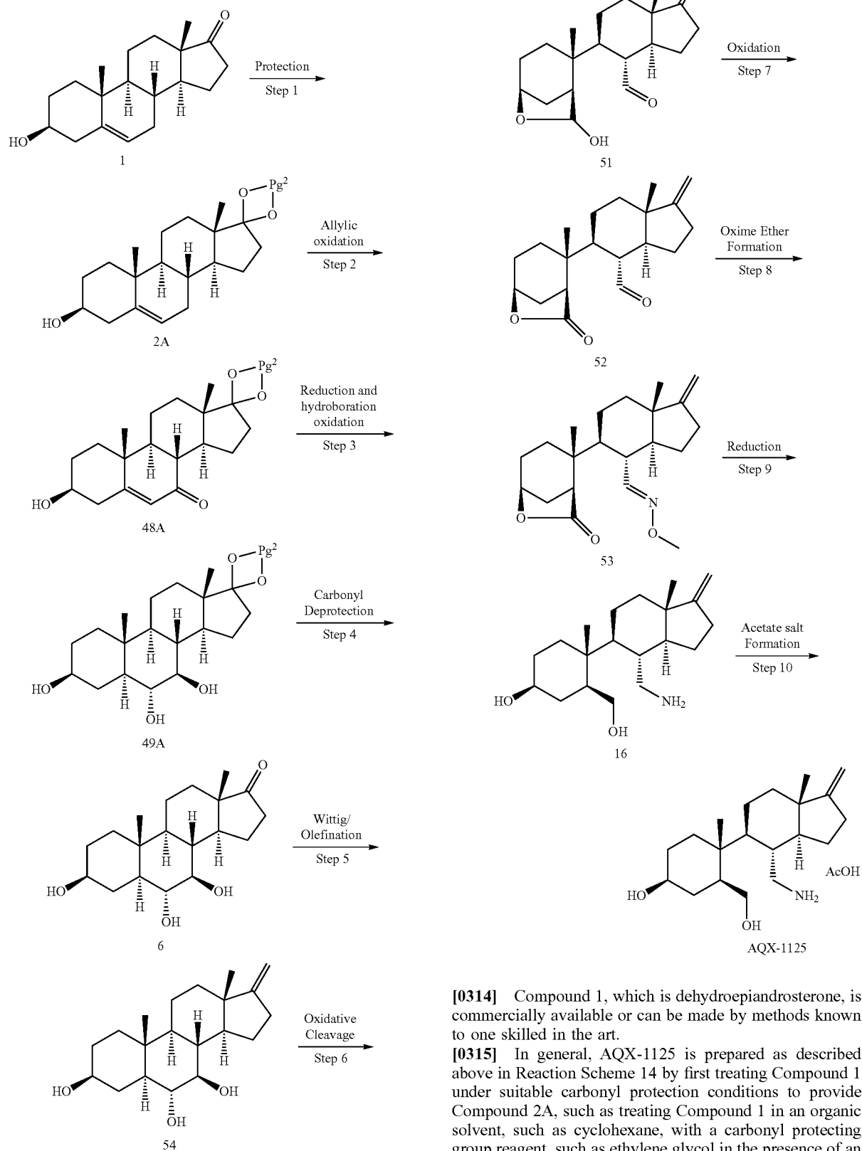
REACTION SCHEME 14
