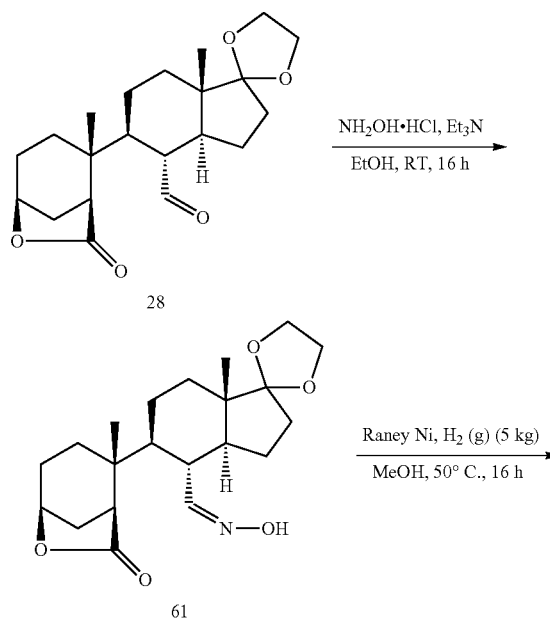
REACTION SCHEME 18:
