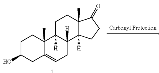
REACTION SCHEME 21
