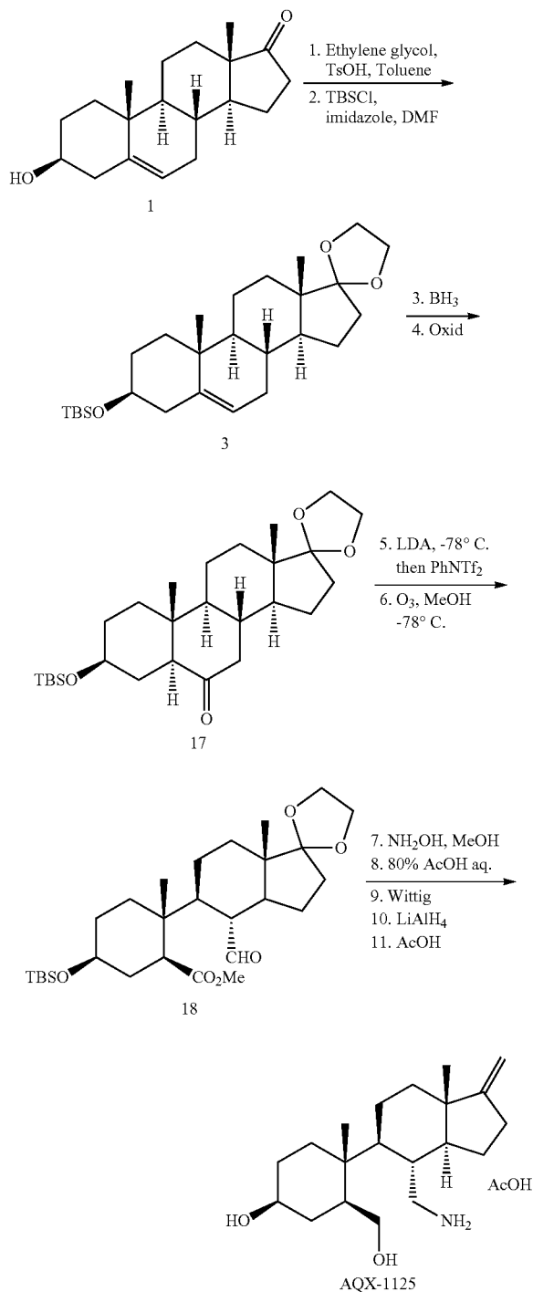
REACTION SCHEME 2 Carbon-carbon bond cleavage by enol triflate ozonolysis
