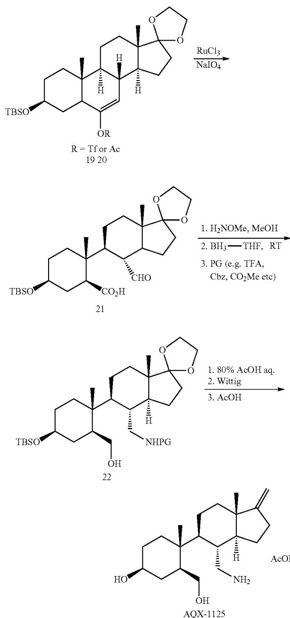
REACTION SCHEME 3
