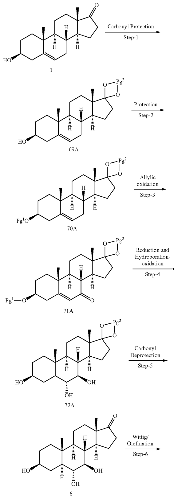
REACTION SCHEME 22
