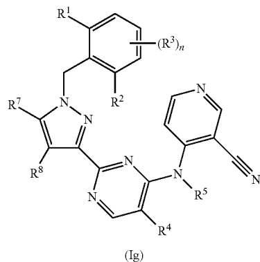
Scheme 7
