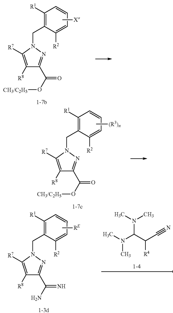
Scheme 13
