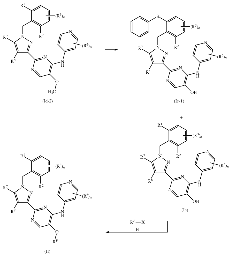
Scheme 6
