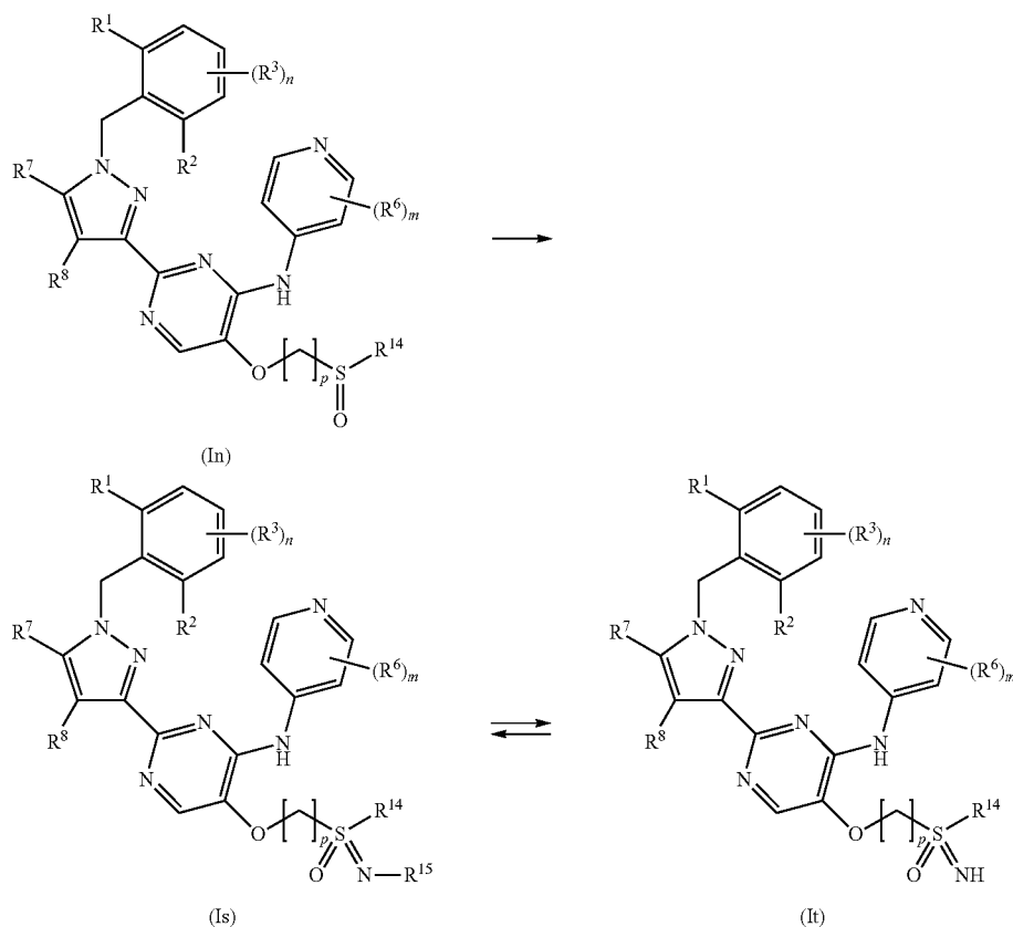
Scheme 17
