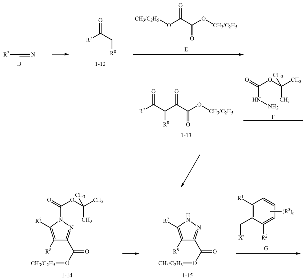
Scheme 4
