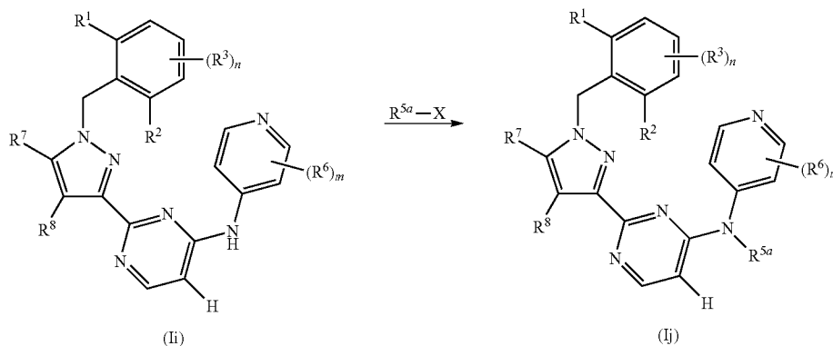
Scheme 9
