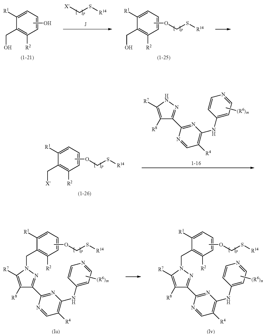
Scheme 18
