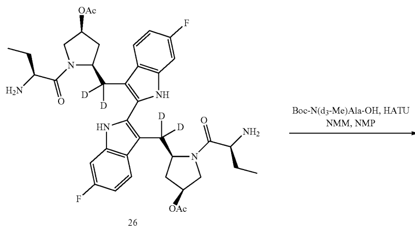
Scheme XXVIII
