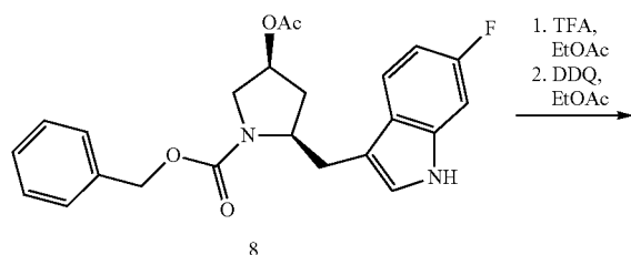
Scheme VIII
