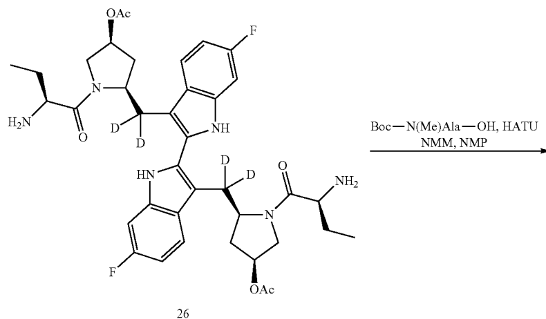
Scheme XXV
