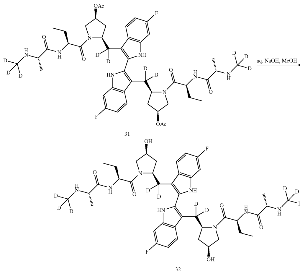
Scheme XXX
