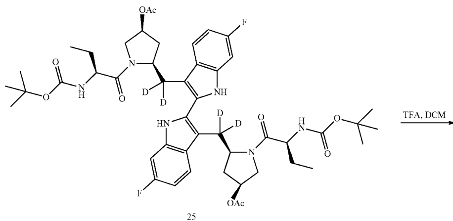
Scheme XXIV
