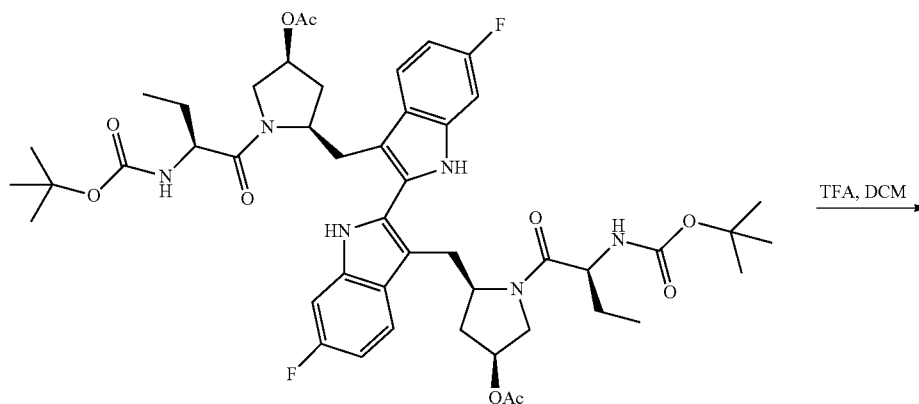
Scheme XI
