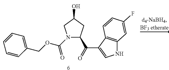
Scheme XIX
