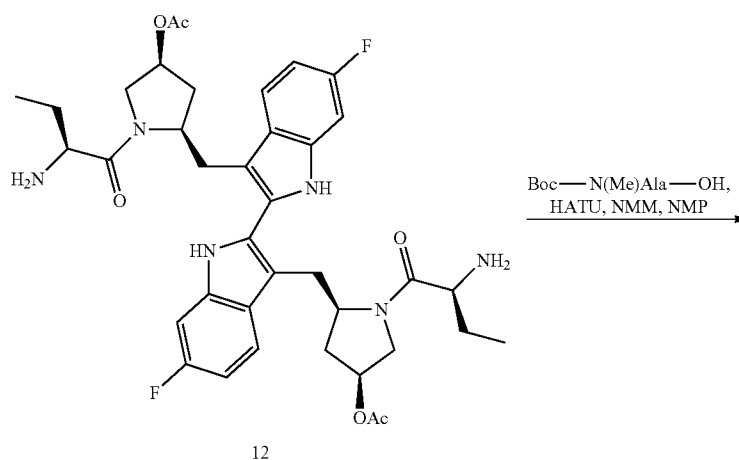
Scheme XII
