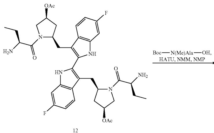
Scheme XVI
