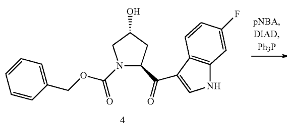
Scheme IV
