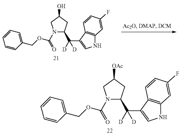
Scheme XX
