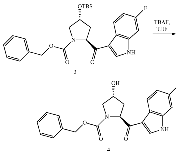
Scheme III
