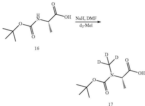
Scheme XV
