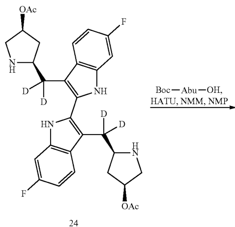
Scheme XXIII
