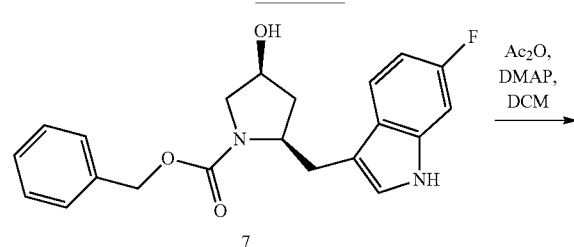
Scheme VII
