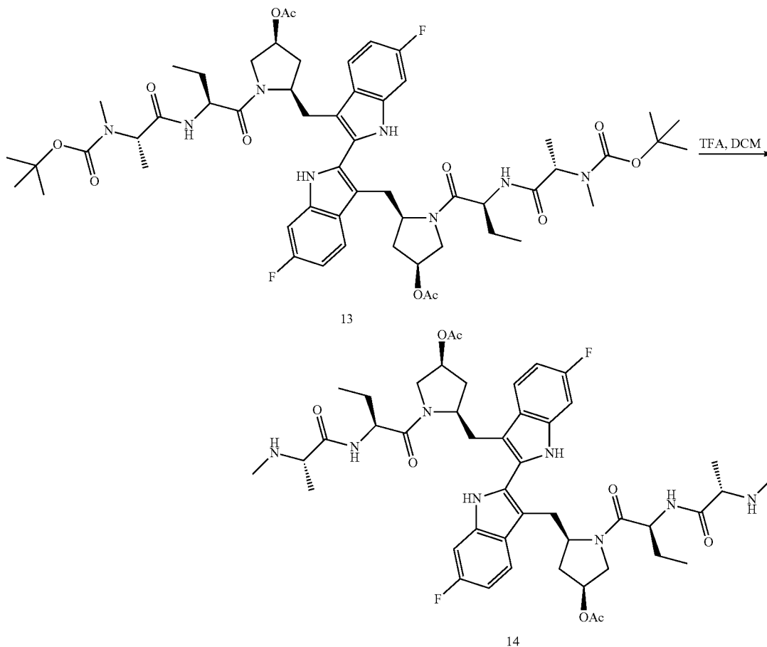
Scheme XIII
