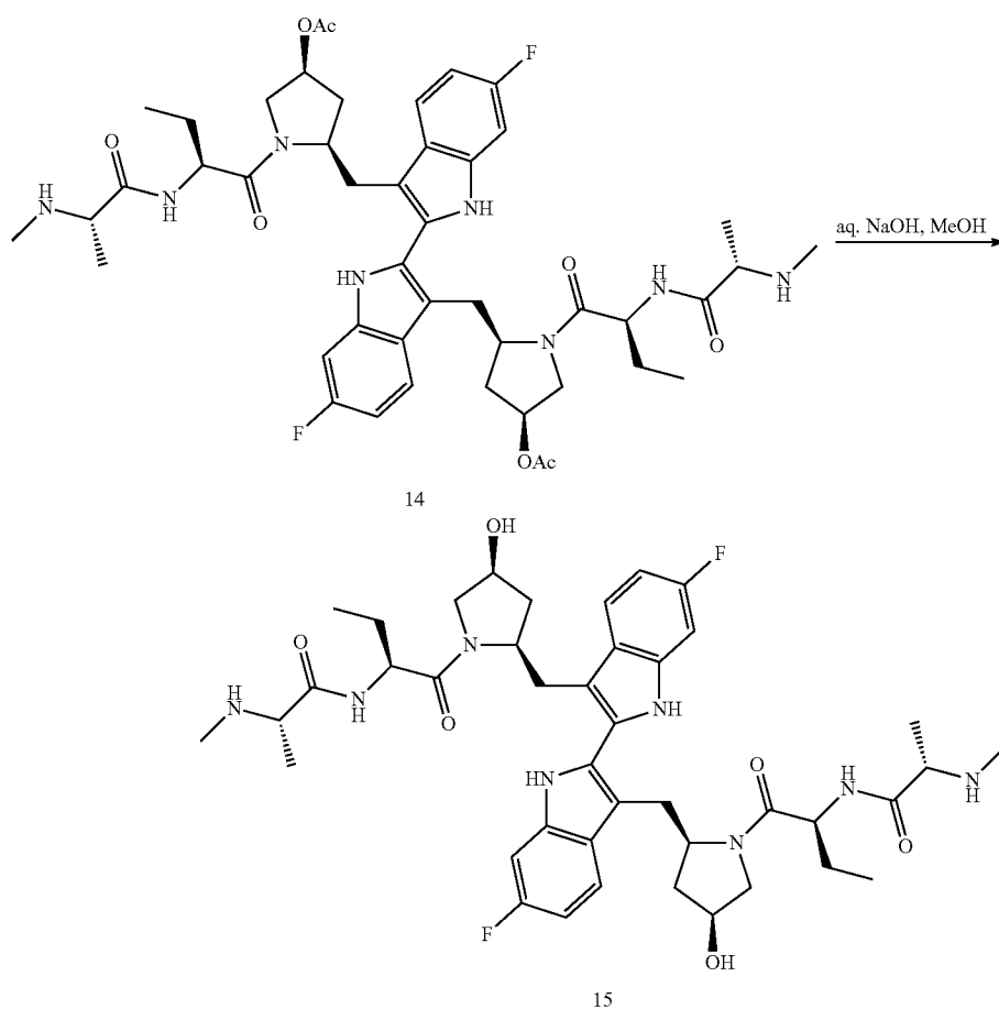
Scheme XIV
