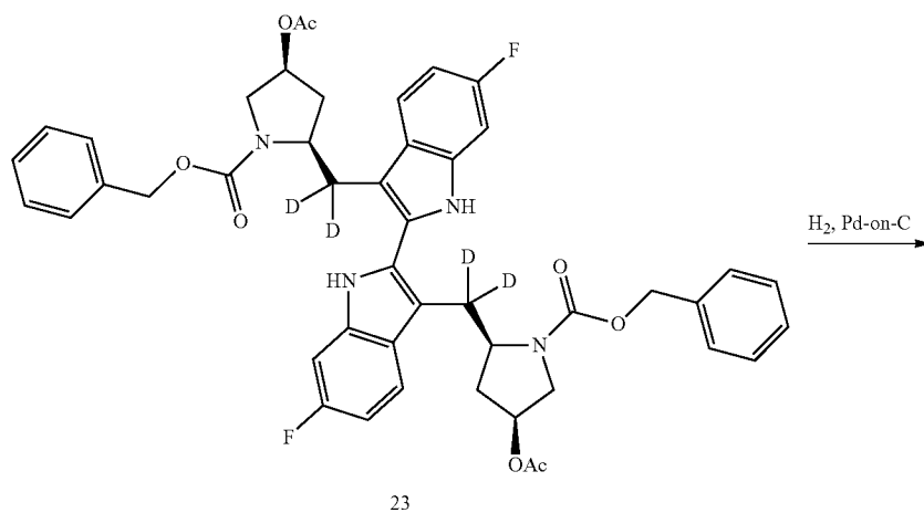
Scheme XXII
