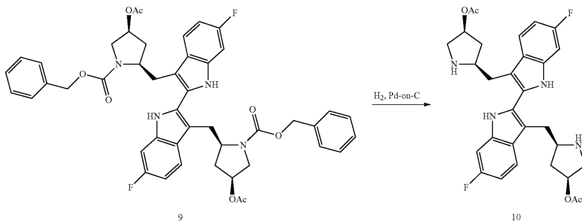
Scheme IX
