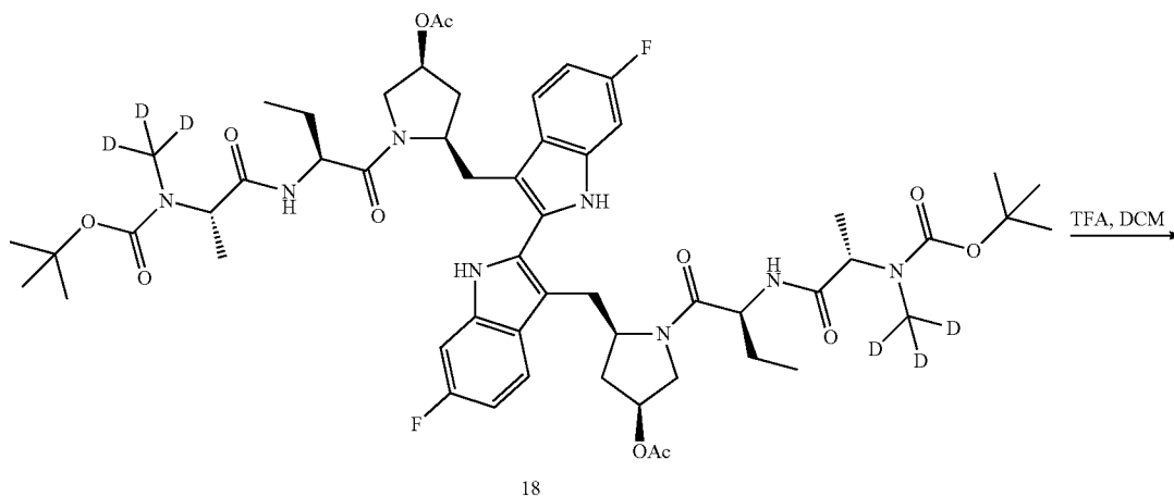
Scheme XVII
