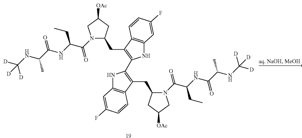
Scheme XVIII
