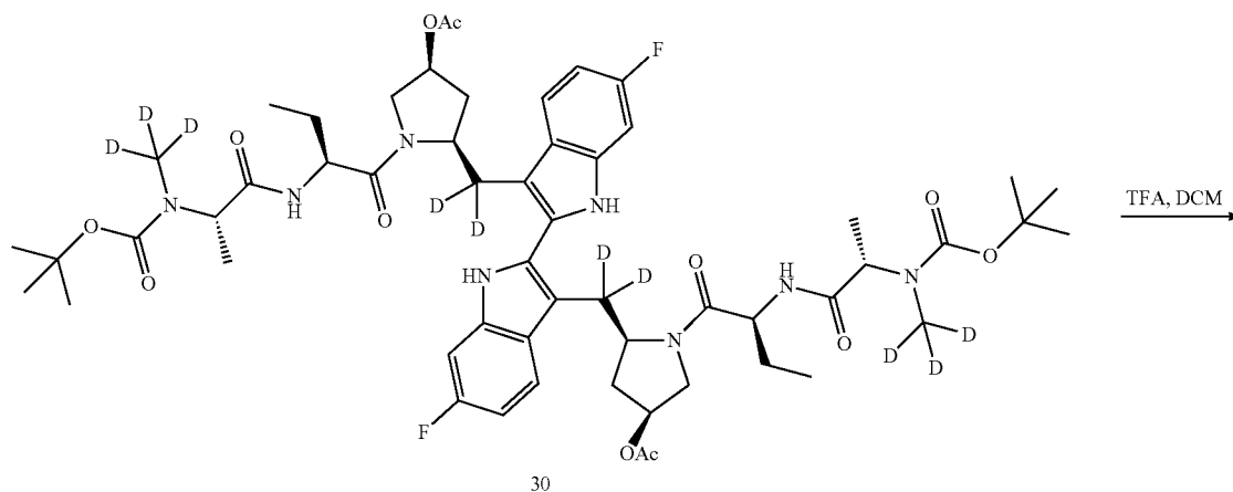
Scheme XXIX
