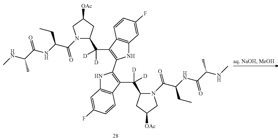
Scheme XXVII
