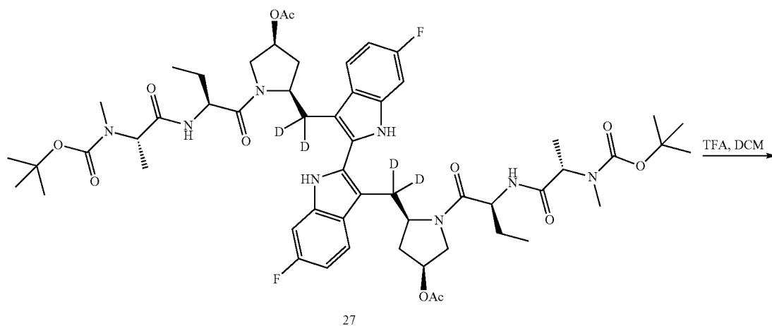
Scheme XXVI
