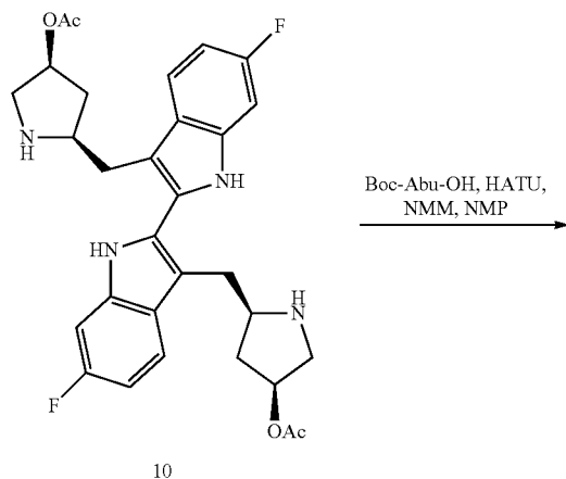
Scheme X
