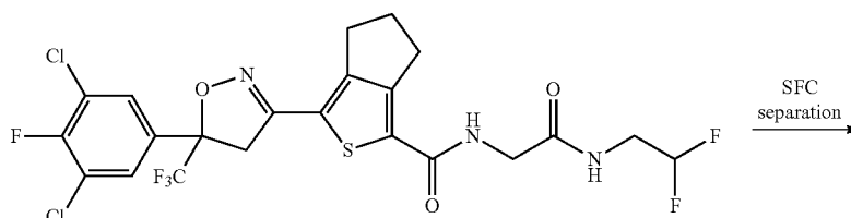
Scheme H SFC Separation of Example 244 to provide S Form
