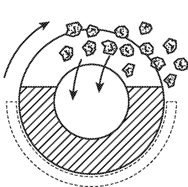
FIG. 13A (PRIOR ART)
