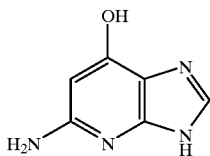
1-deaza-Guanine
