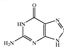
8-Aza-Guanine
