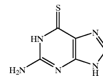
6-Thio guanine
