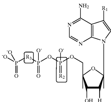
7-Substituted-7-Deaza-dATP
