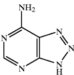
8-aza-Adenine
