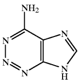
2-aza-Adenine
