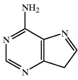
9-deaza-Adenine
