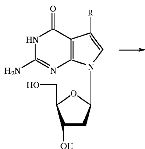
7-deaza-2'-deoxyguanosine
