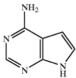
7-deaza-Adenine
