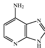
1-deaza-Adenine
