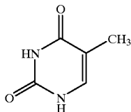
Thymine
