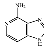
3-deaza-Adenine
