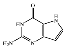
9-deaza-Guanine
