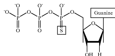
■ - Thiophosphate
