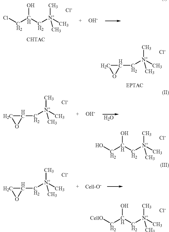
Scheme 1. Cationization of Cellulose and Hydrolysis of EPTAC
