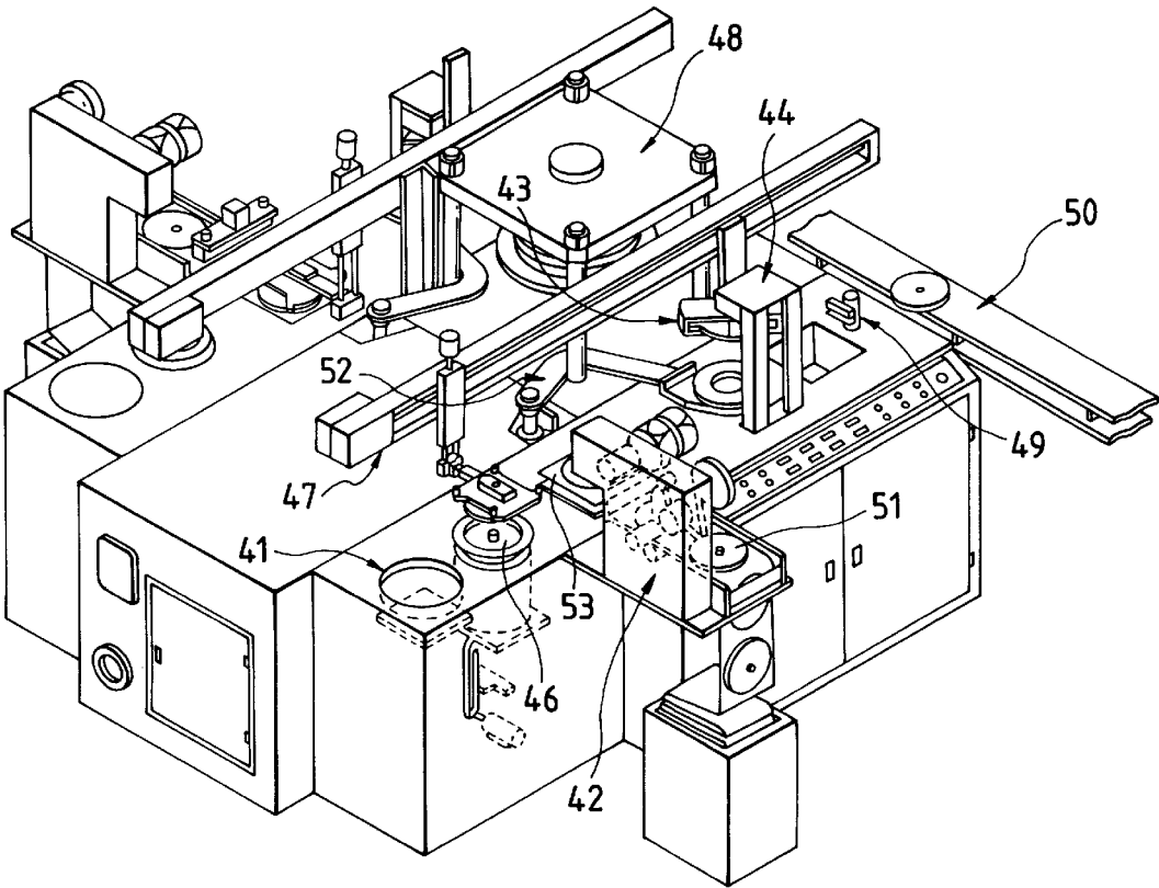
FIG. 16 PRIOR ART
