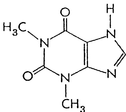
Theophylline
