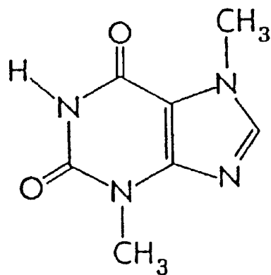
Theobromine
