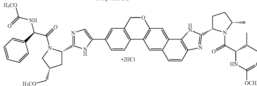
Compound (A-a)
