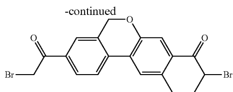
Compound (I-a)
