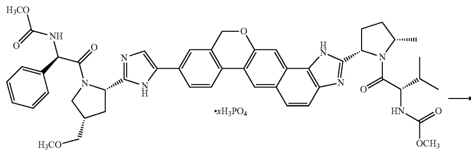
Compound (A-b)
