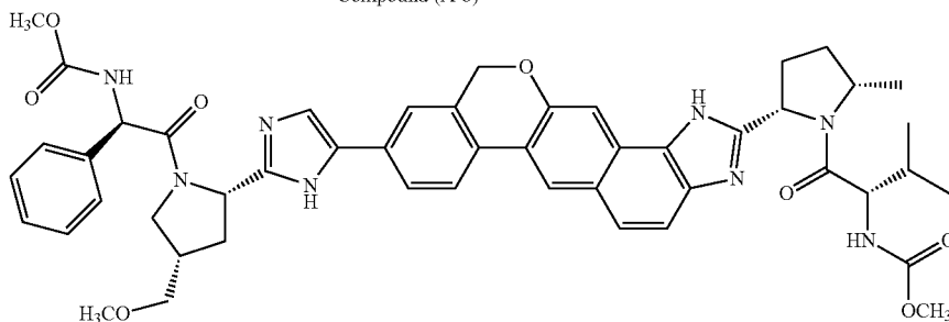
Compound (A)
