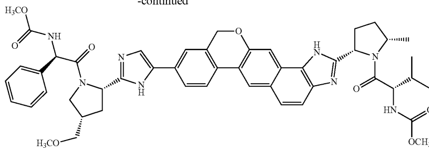
Compound (A)
