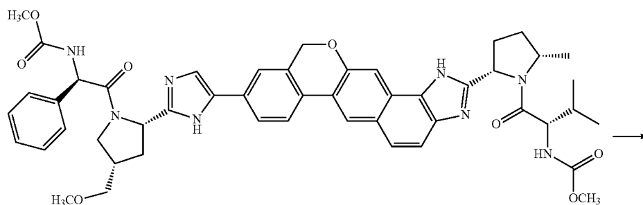
Compound (A)
