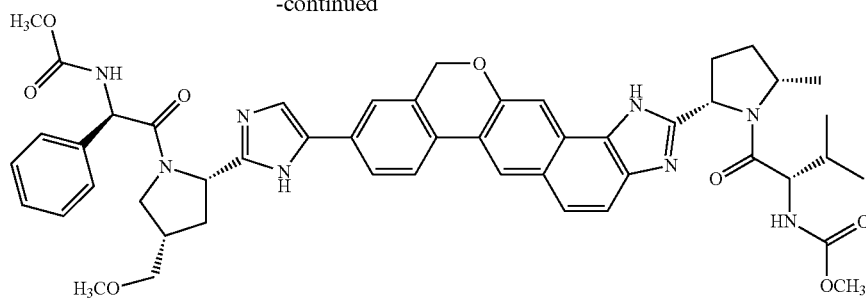
Compound (A)
