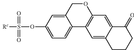
Compound (5-9)
