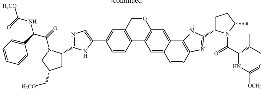
Compound (A)
