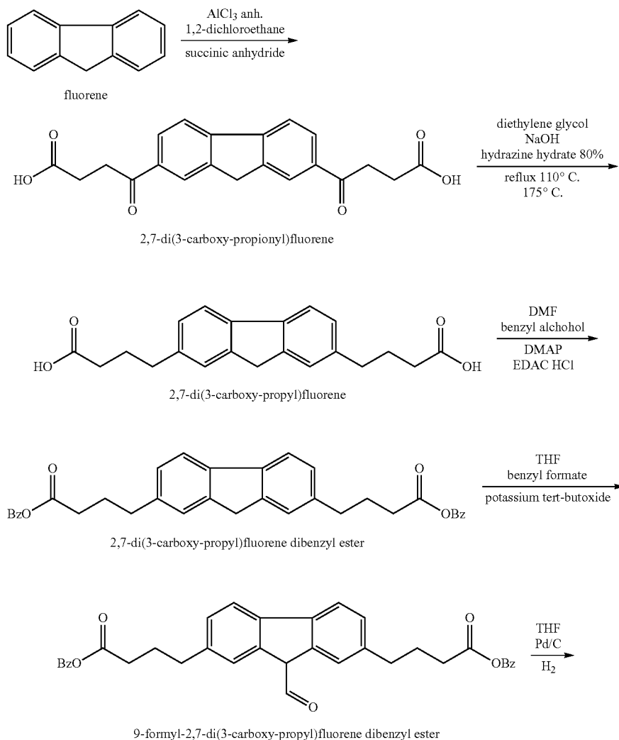
Scheme 6.
