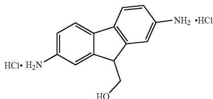
9-hydroxymethyl-2,7-diaminofluorene dihydrochloride
