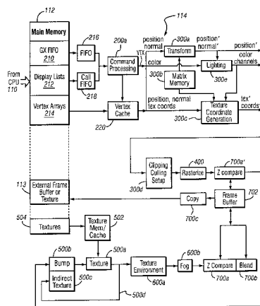
EXAMPLE GRAPHICS PROCESSOR FLOW
