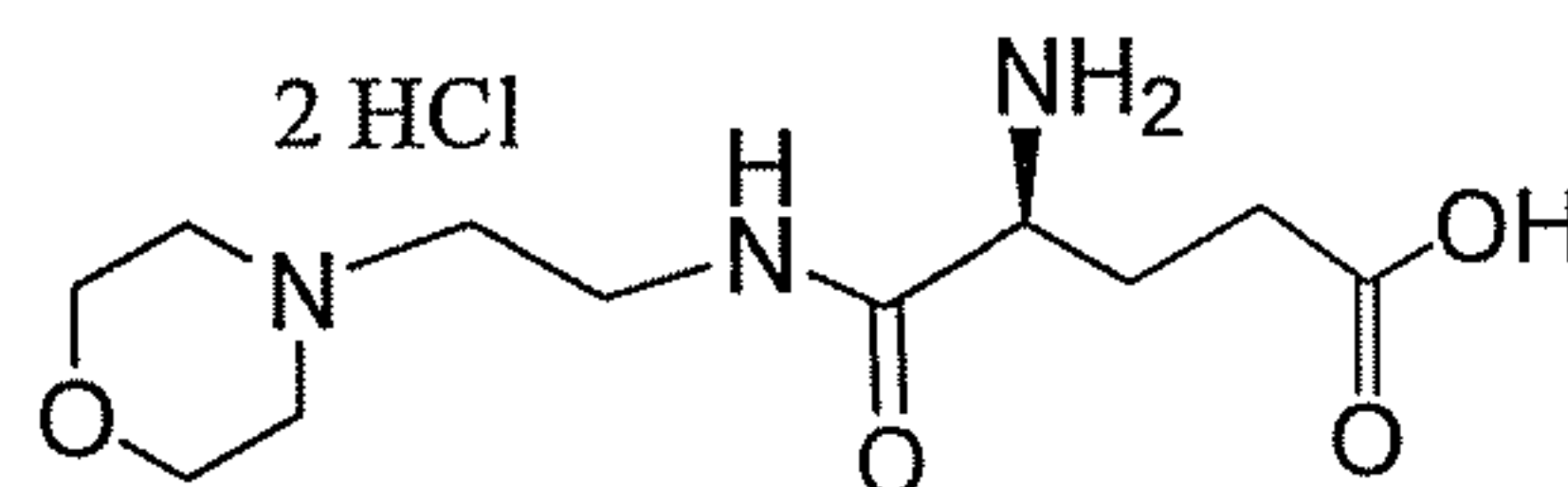
Compound 17
