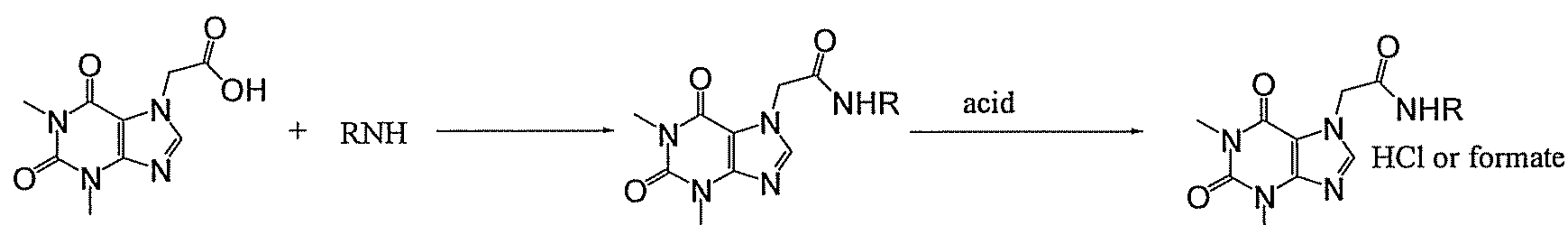
Scheme 2
