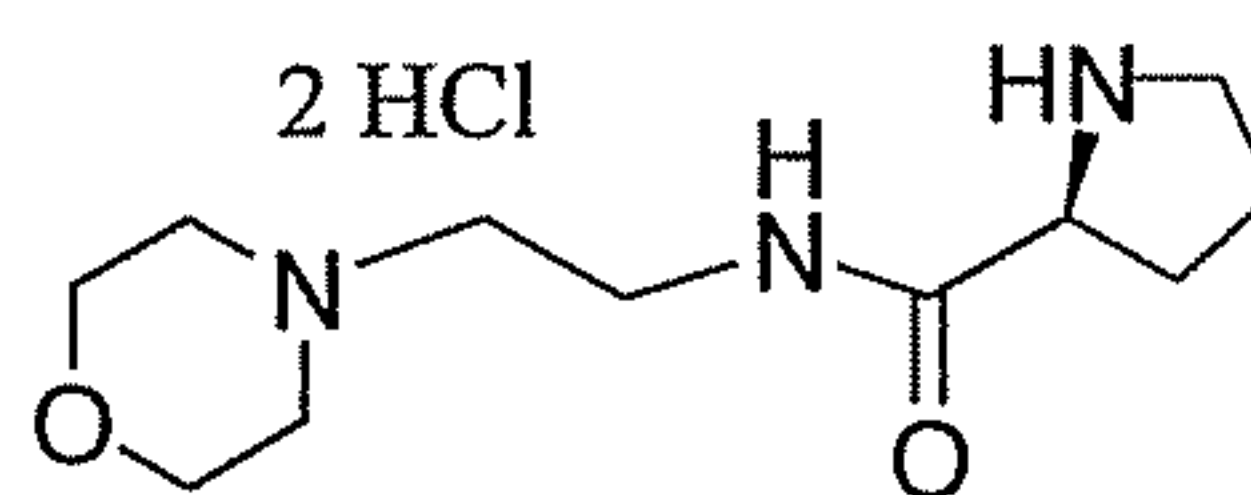
Compound 18
