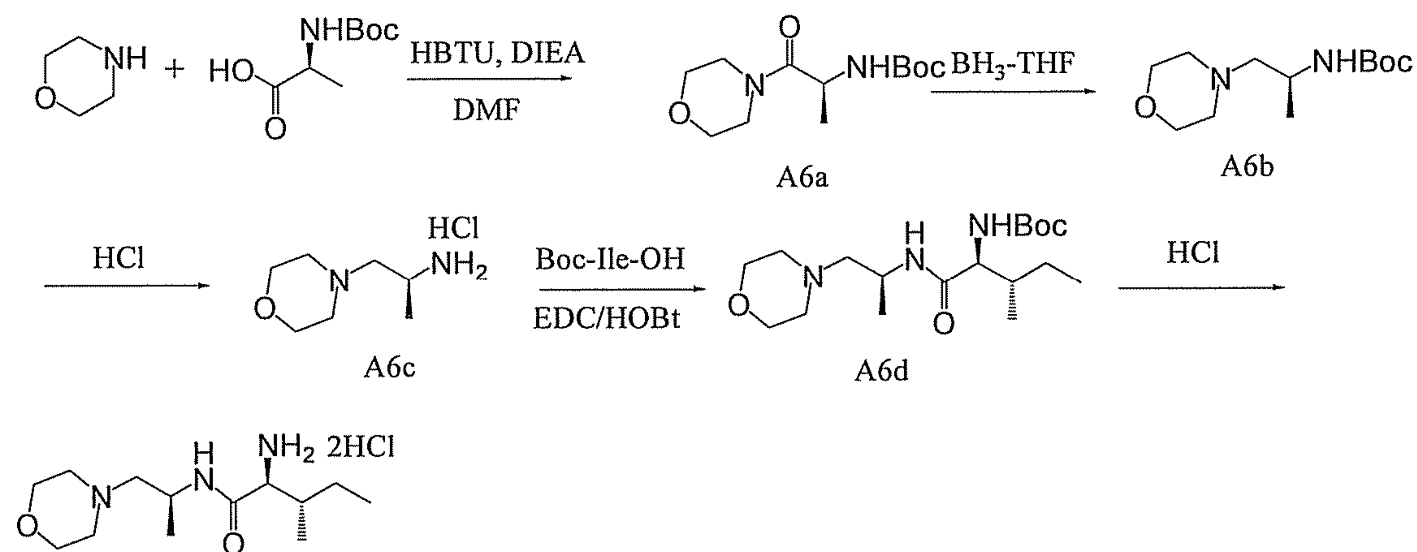
Compound 6
