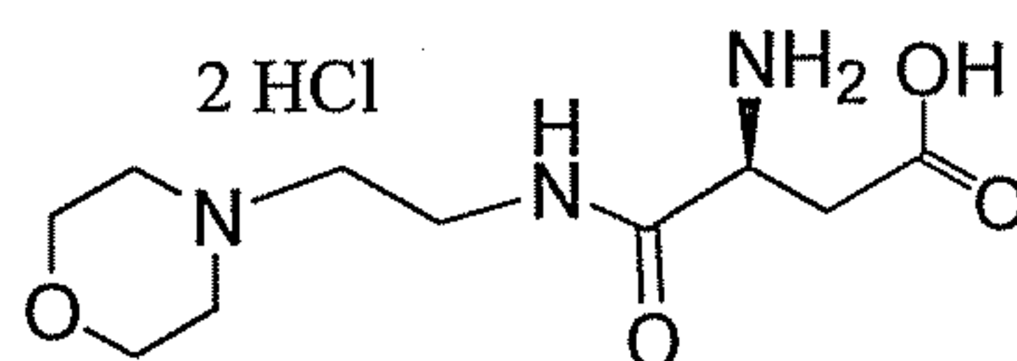
Compound 16
