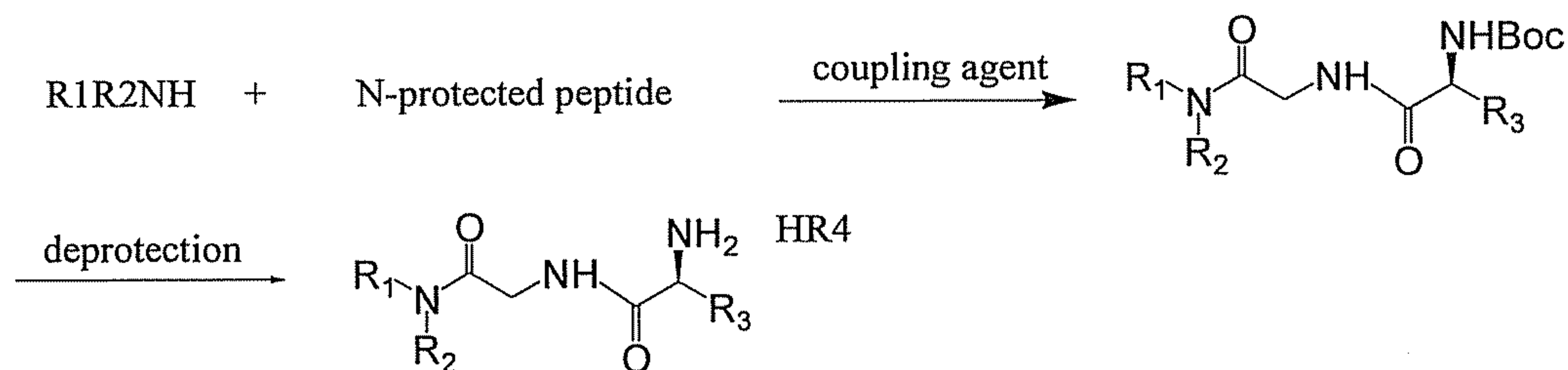
Scheme 1
