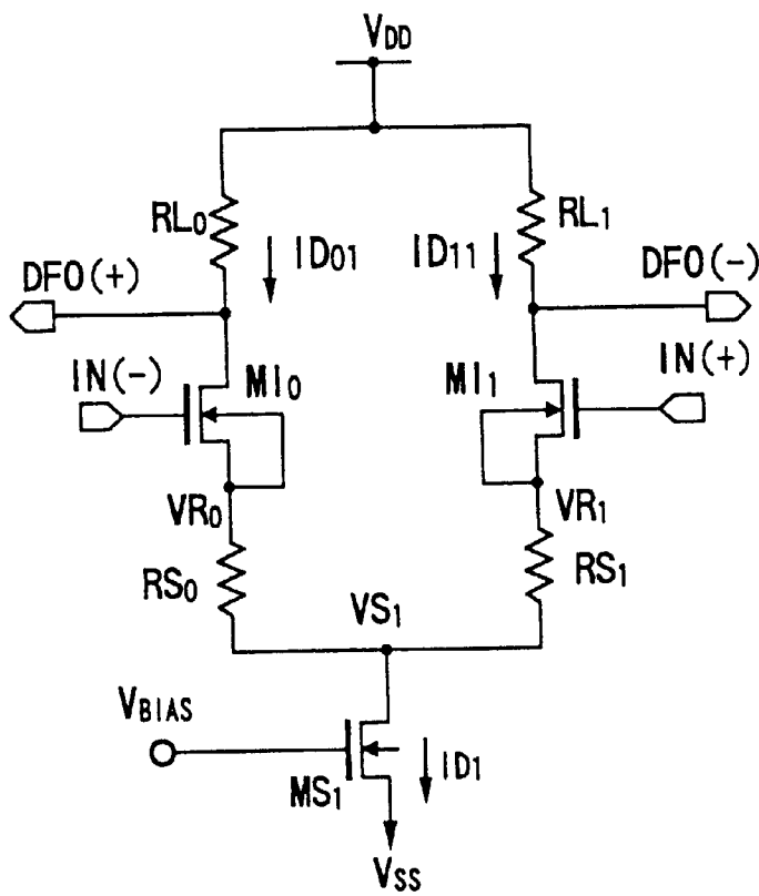
PRIOR ART FIG.3
