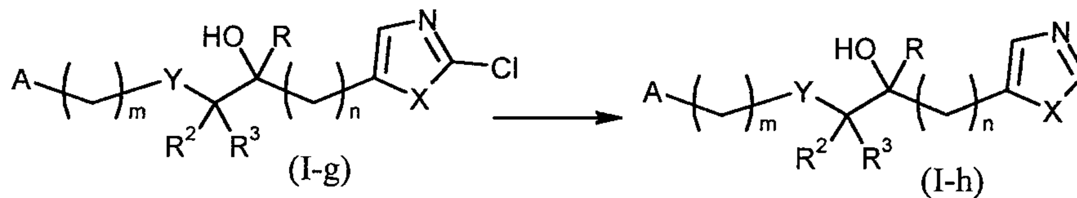
Scheme 6 Process F
