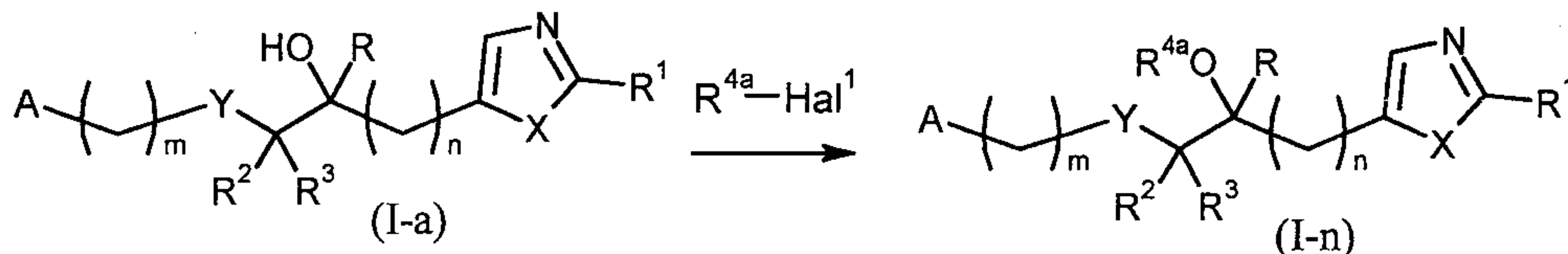
Scheme 10 Process J
