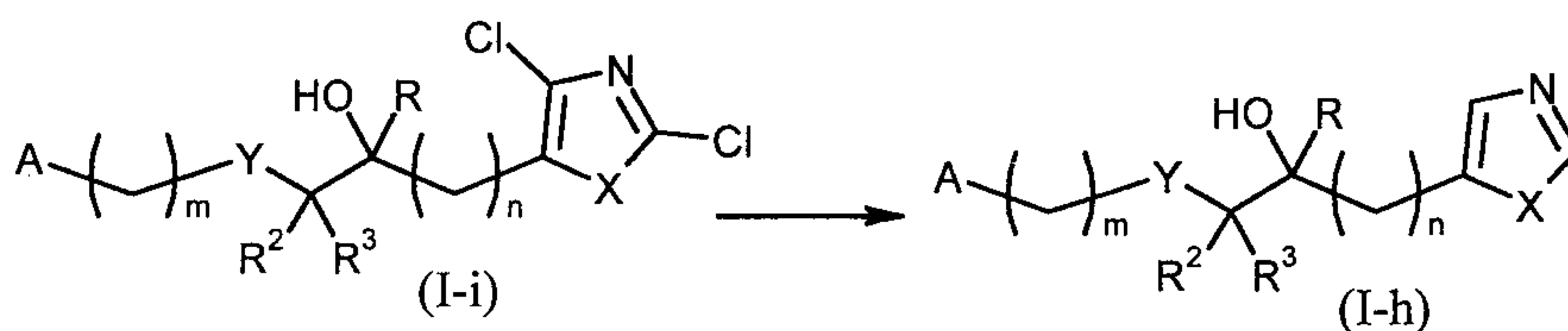
Scheme 7 Process G
