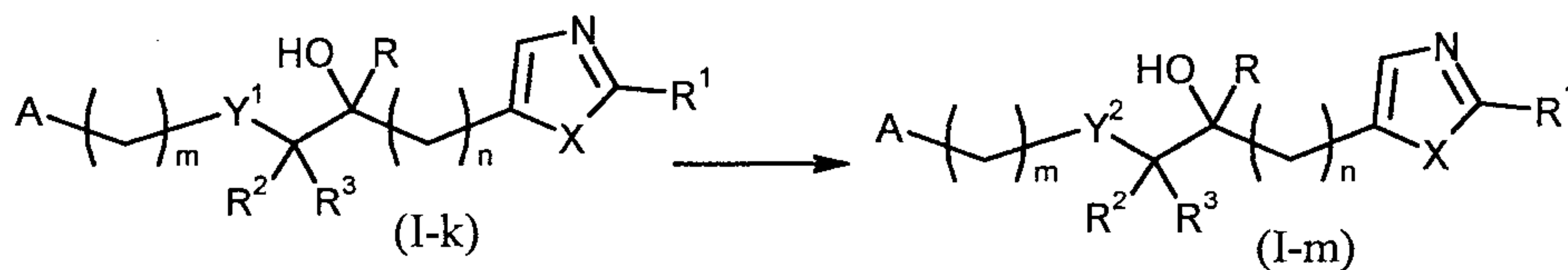
Scheme 9 Process I
