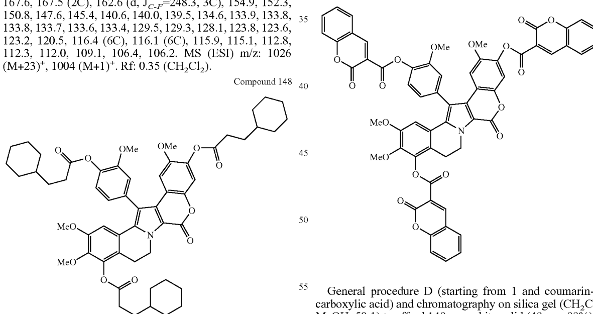
Compound 149
