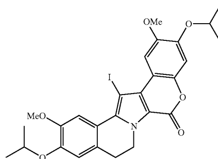
Compound 189
