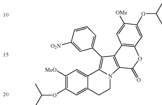
Compound 217
