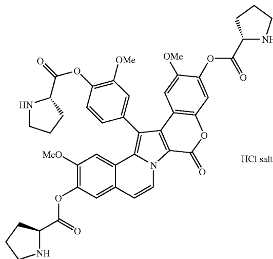
Compound 180
