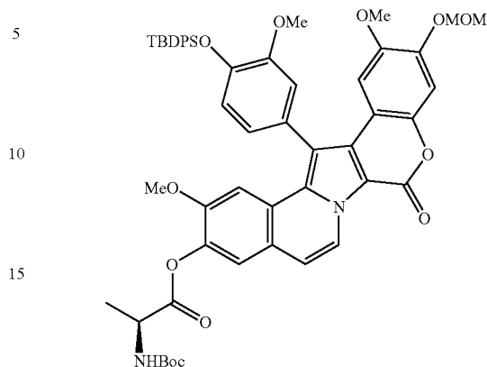
Compound 234
