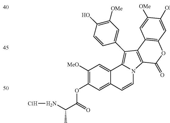
Compound 239
