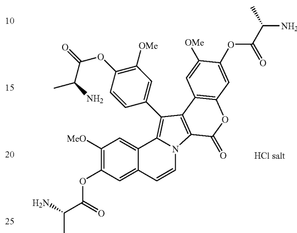
Compound 199
