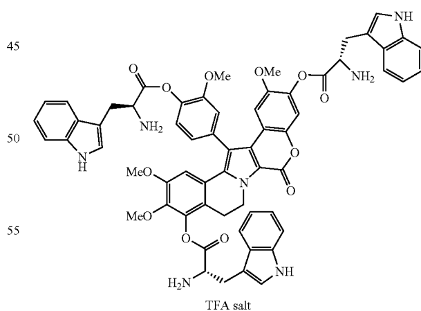
Compound 132
