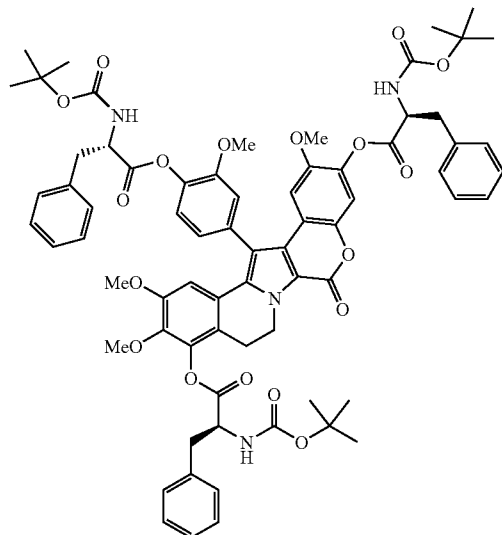
Compound 125
