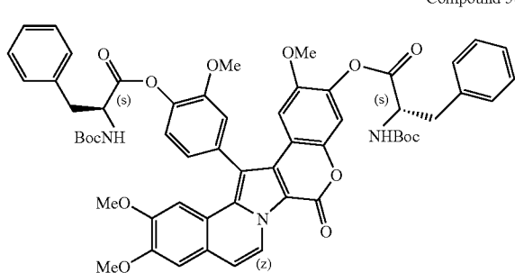
Compound 58
