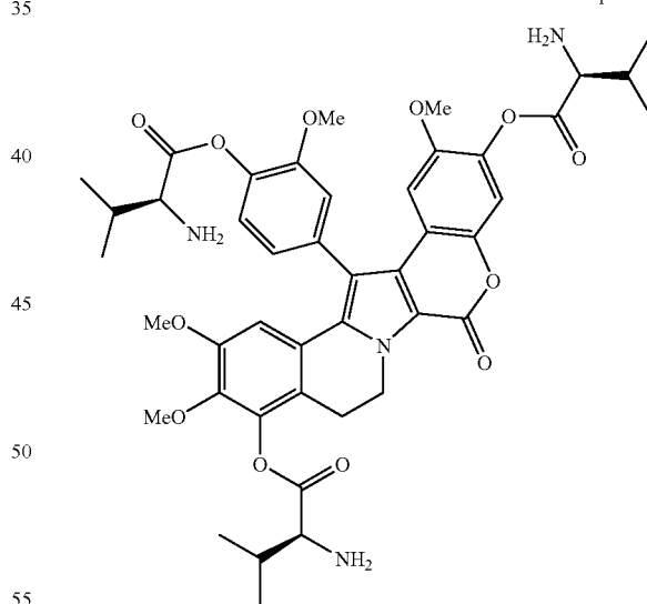
TFA salt
