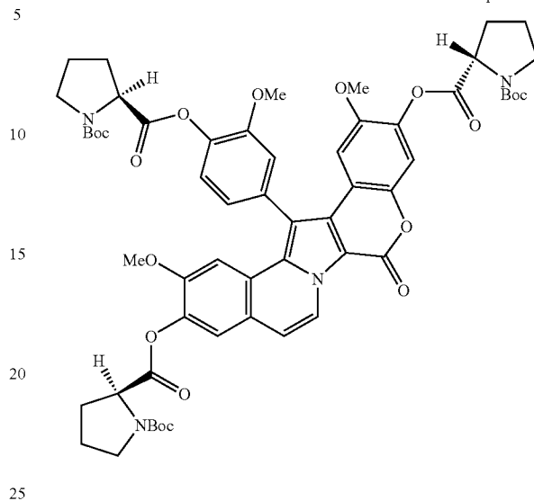
Compound 127
