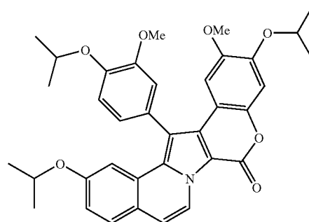
Compound 179
