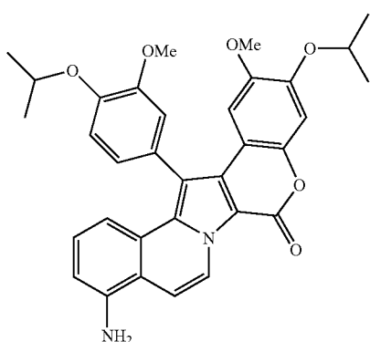
Compound 178
