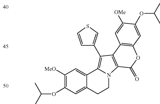
Compound 218
