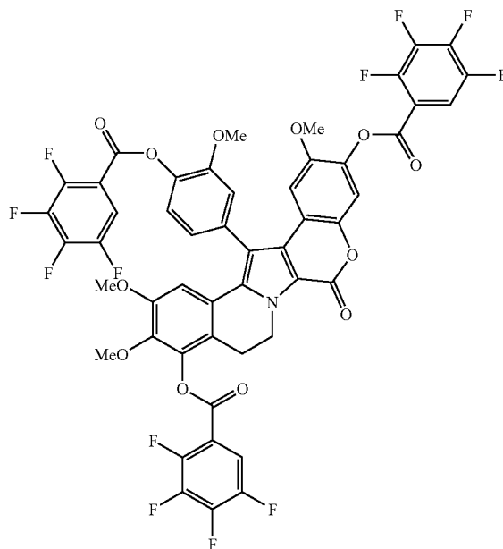
Compound 99
