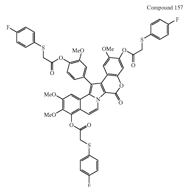
Compound 157
