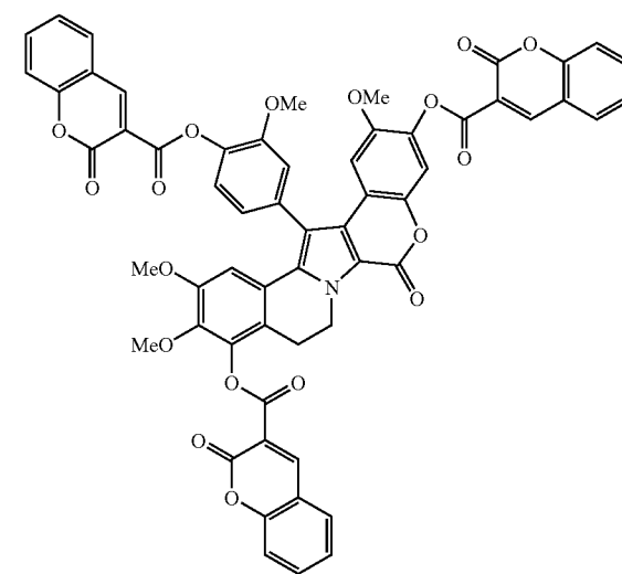
Compound 149
