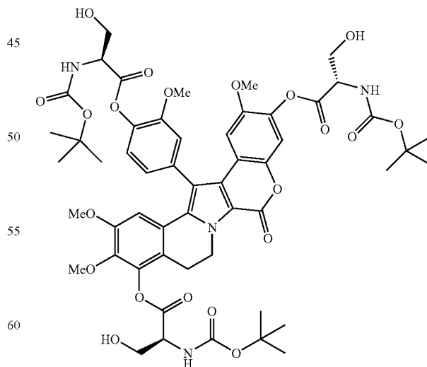
Compound 60
