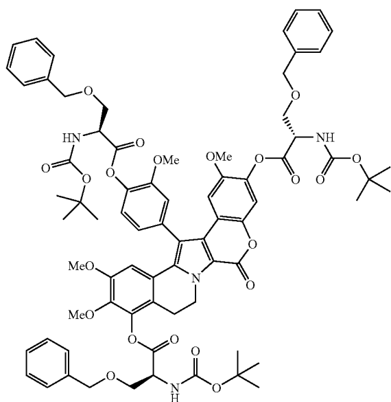
Compound 68
