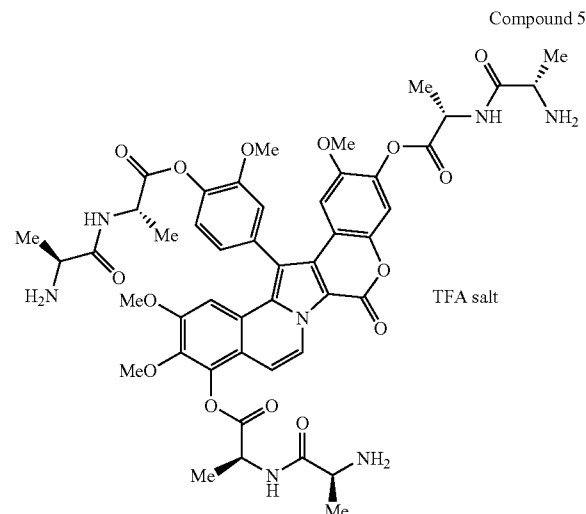
Compound 5
