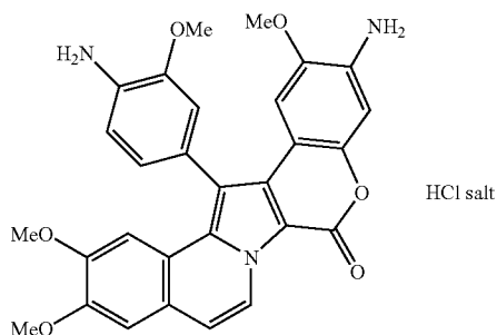
Compound 170
