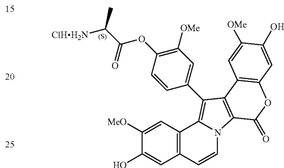
Compound 238
