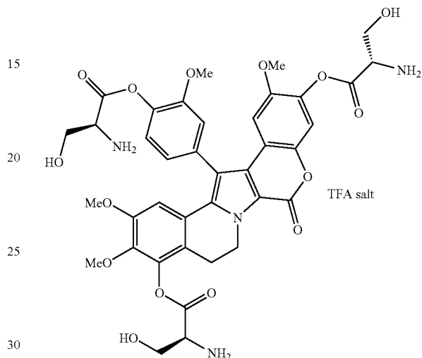
Compound 59
