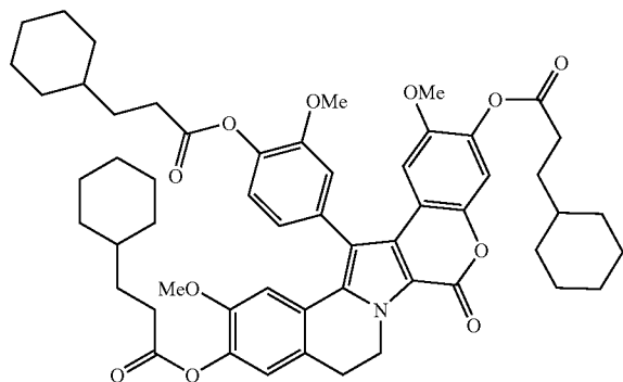
Compound 106
