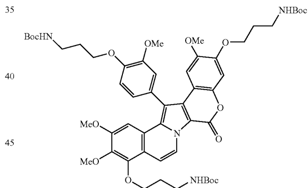
Compound 200
