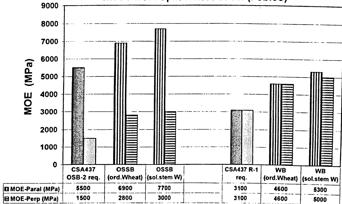
Fig.3 Modulus of Elasticity (MOE) of OSSB and Waferboard made from Split Wheat Straw (Feb.98)
