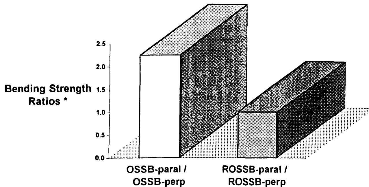
Fig.1 Bending Strength ratios "Parallel/Perpendicular" for Composites Boards made with Oriented Straw Strands (OSSB) and Random Oriented Straw Strands (ROSSB) (using Wheat Straw Strands of length 1" - 4")
