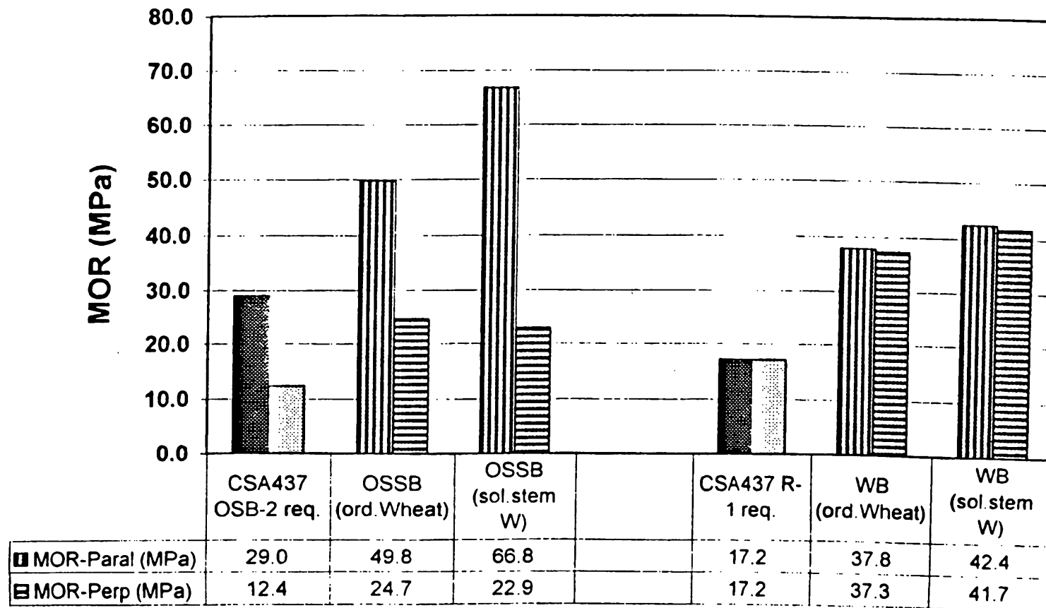
Fig.4 Bending Strength (MOR) of OSSB and Waferboard made from Split Wheat Straw (Feb.98)
