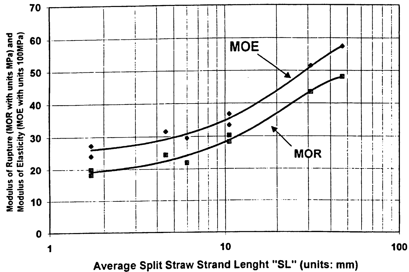
Fig. 2 Average Split Straw Strand Length and observed Bending Properties of straw panels
