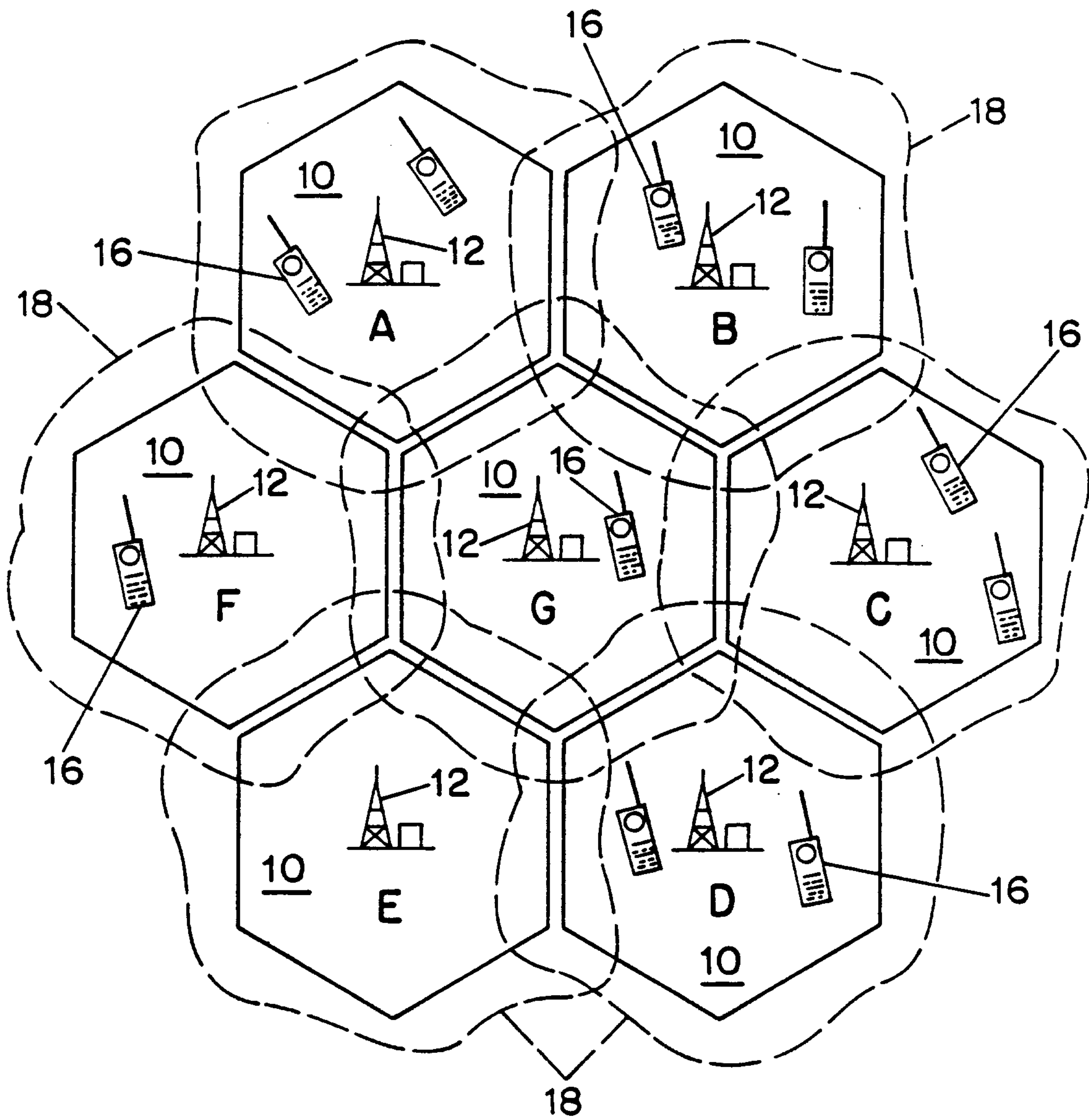
FIG. 1 (PRIOR ART)
