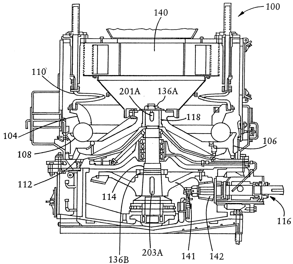
FIG. 1 PRIOR ART
