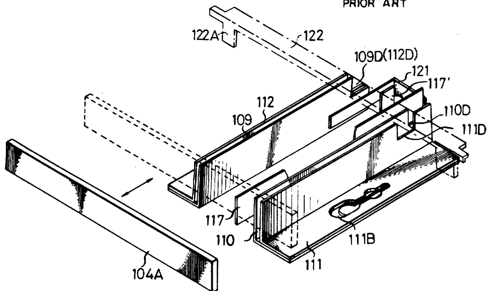
FIG.8 PRIOR ART
