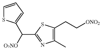
4-Methyl-5-(2-nitrooxy-ethyl)-2-(nitrooxy-thiophen-2-yl-methyl)-thiazole (Pet-95);
