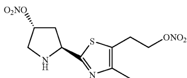
4-Methyl-5-(2-nitrooxy-ethyl)-2-(4-nitrooxy-pyrrolidin-2-yl)-thiazole (Pet 93);
