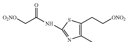
N-[4-Methyl-5-(2-nitrooxy-ethyl)-thiazol-2-yl]-2-nitroxy-acetamide (Pet 96);
