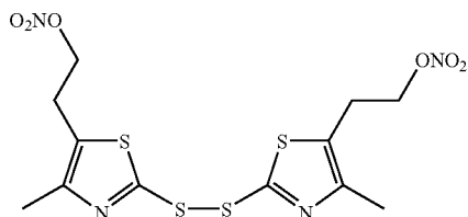
Bis-[4-methyl-5-(2-nitrooxy-ethyl)-thiazol-2-yl]-disulfide (Pet-54);
