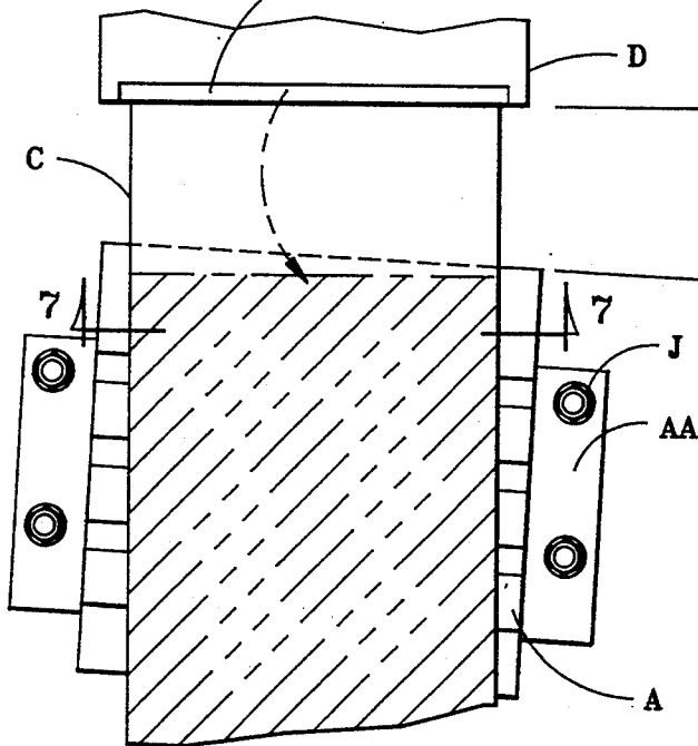
FIG. 6 PRIOR ART
