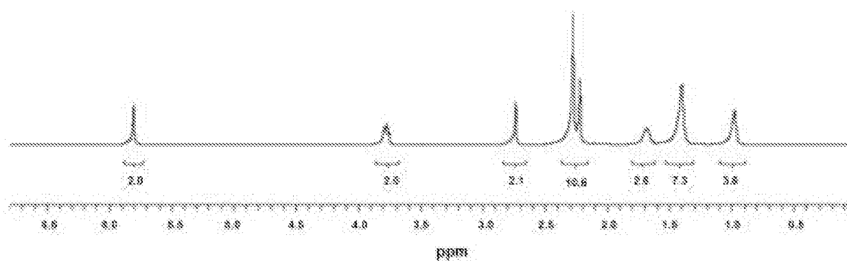
Fig. 2. ^1\text{H} NMR spectrum, 400 MHz in \text{CDCl}_3 , of 1-hexyl-2,5-dimethyl-1H-pyrrole
