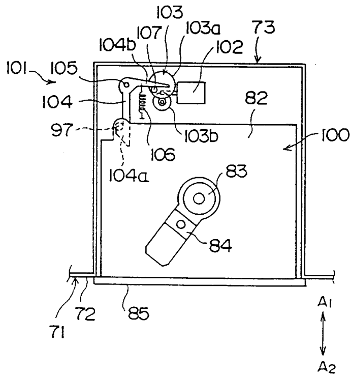
FIG. 2 (PRIOR ART)
