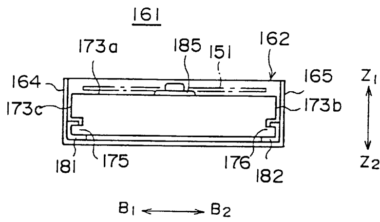
FIG. 4 (PRIOR ART)
