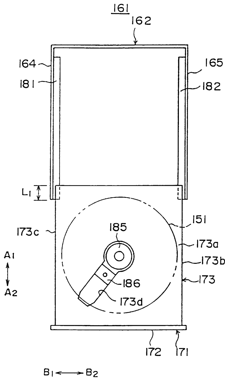
FIG. 3 (PRIOR ART)
