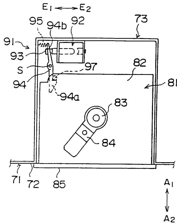
FIG. 1 (PRIOR ART)
