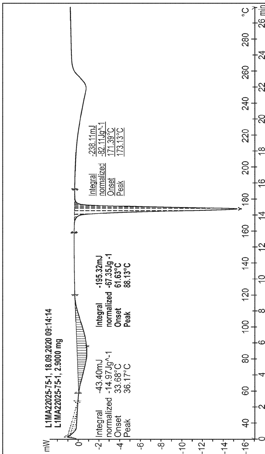
FIG. 9C DSC thermogram of Compound (I) free base Form FB-A-0 from 4– 40 °2θ.
