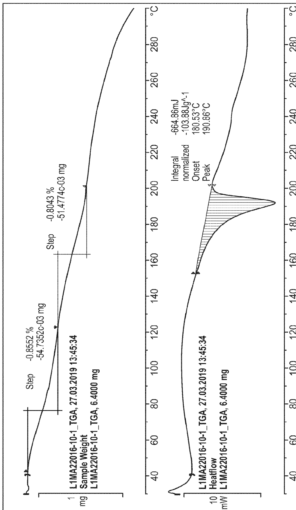
FIG. 4B TGA and DSC thermograms of Compound (I) besylate Form 1-A.
