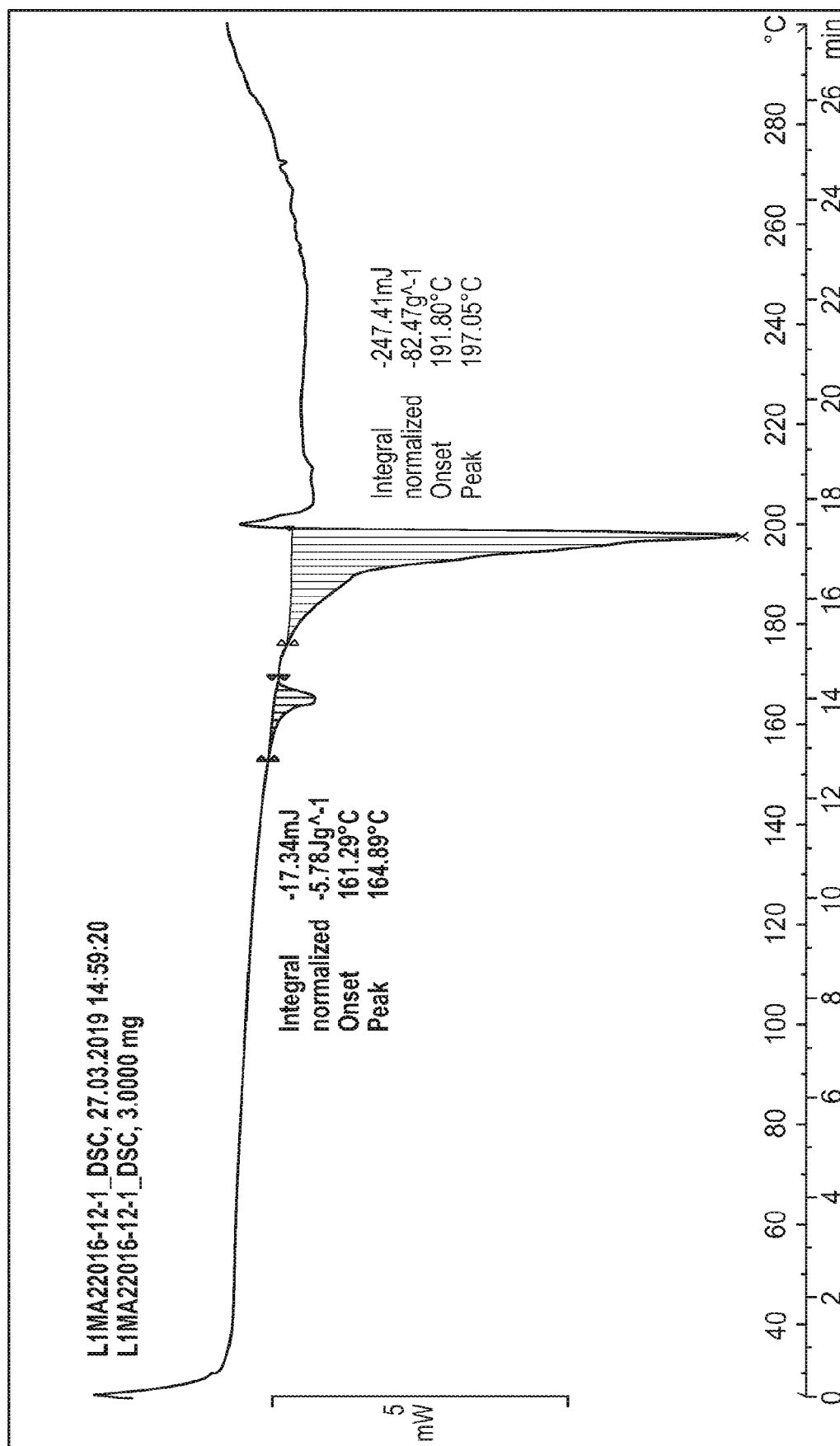
FIG. 1C DSC thermogram of Compound (I) phosphate Form A.
