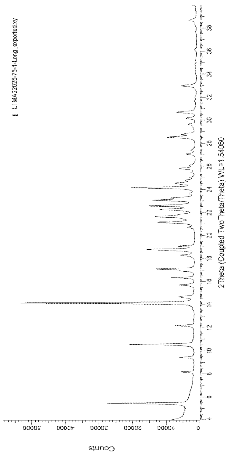
Figure 9A- XRPD diffractogram of Compound (I) free base Form FB-A-0 from 4-40 °2θ.
