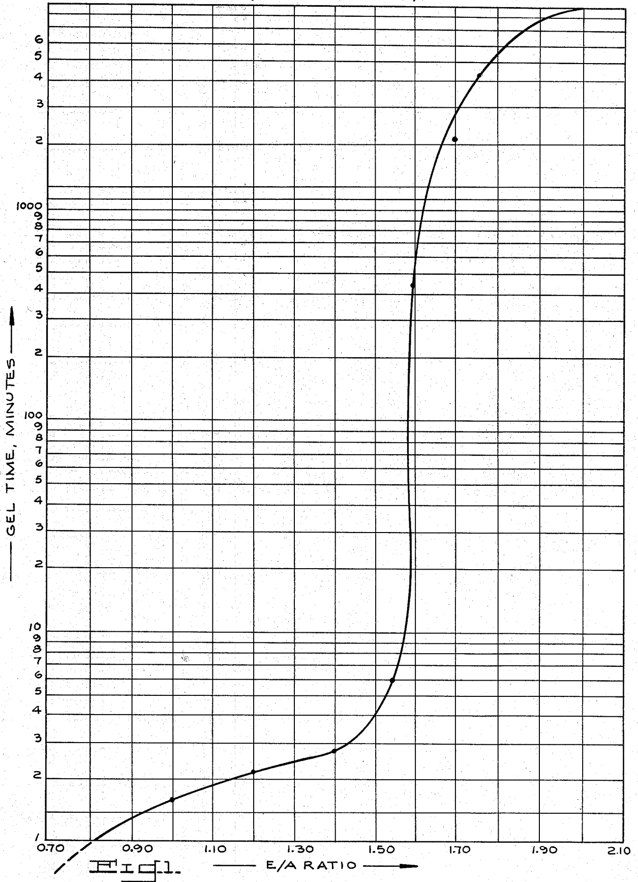
GEL TIME VS. E/A RATIO N 2 O 2 ACTIVATED 10% POLY(NMDAA-HCL SALT) EPI RESINS
