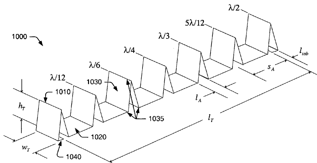
FIG. 10B FOLDED PATTERN
