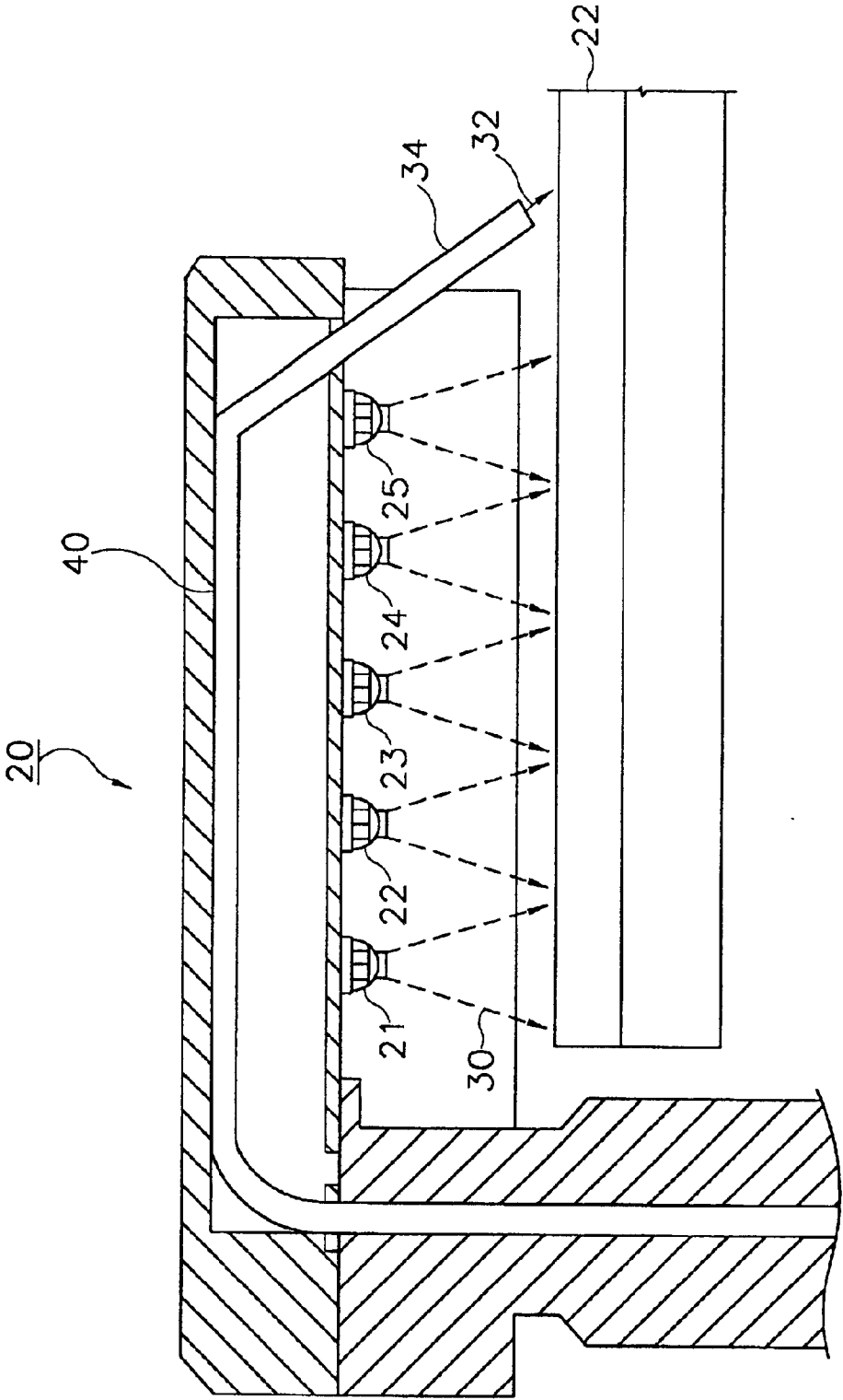
FIG. 2 (PRIOR ART)
