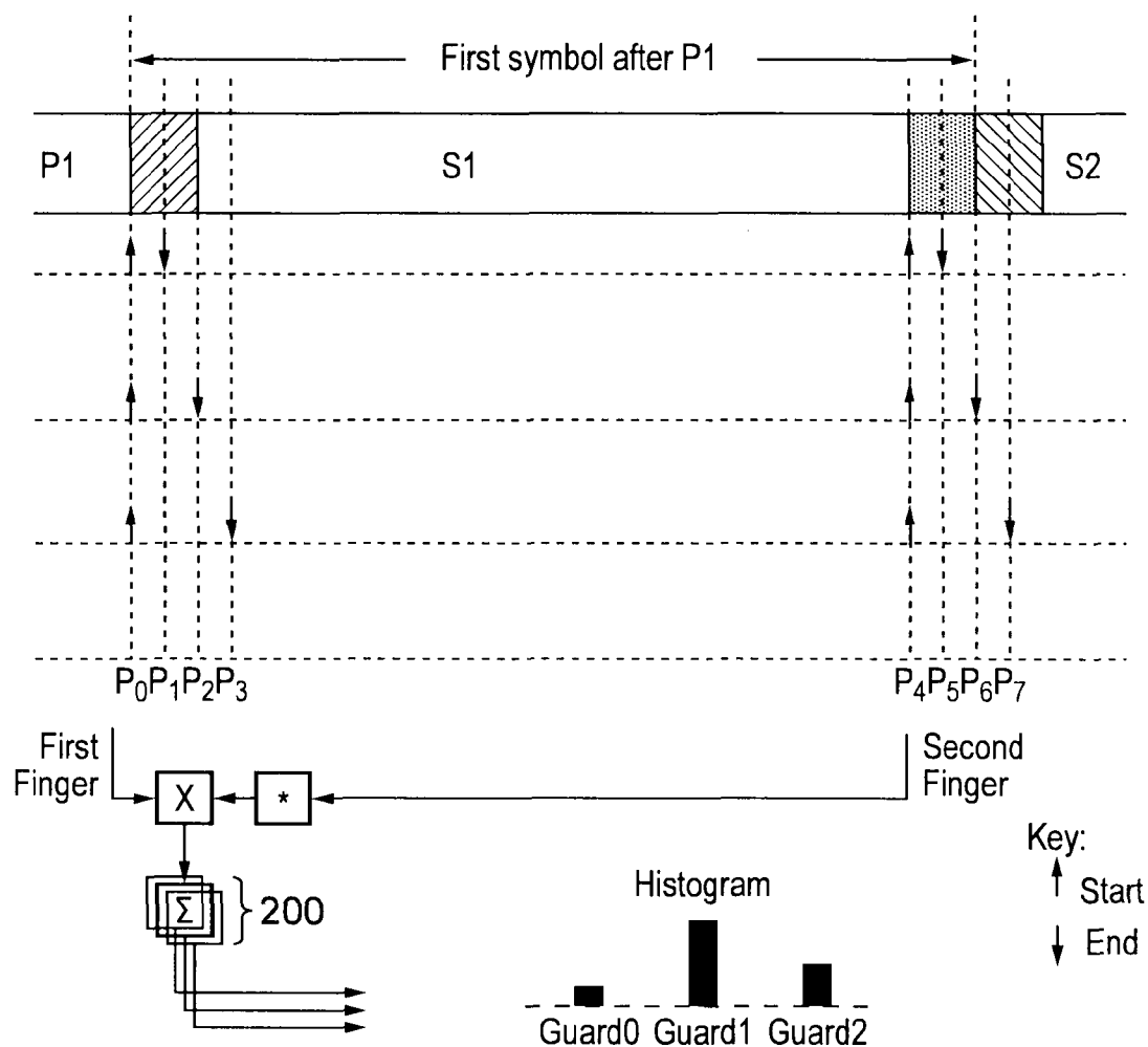
Operation of Simplified Architecture at First Symbol
