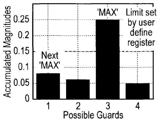
'Accumulated Correlation Magnitudes' for Possible Guard Intervals
