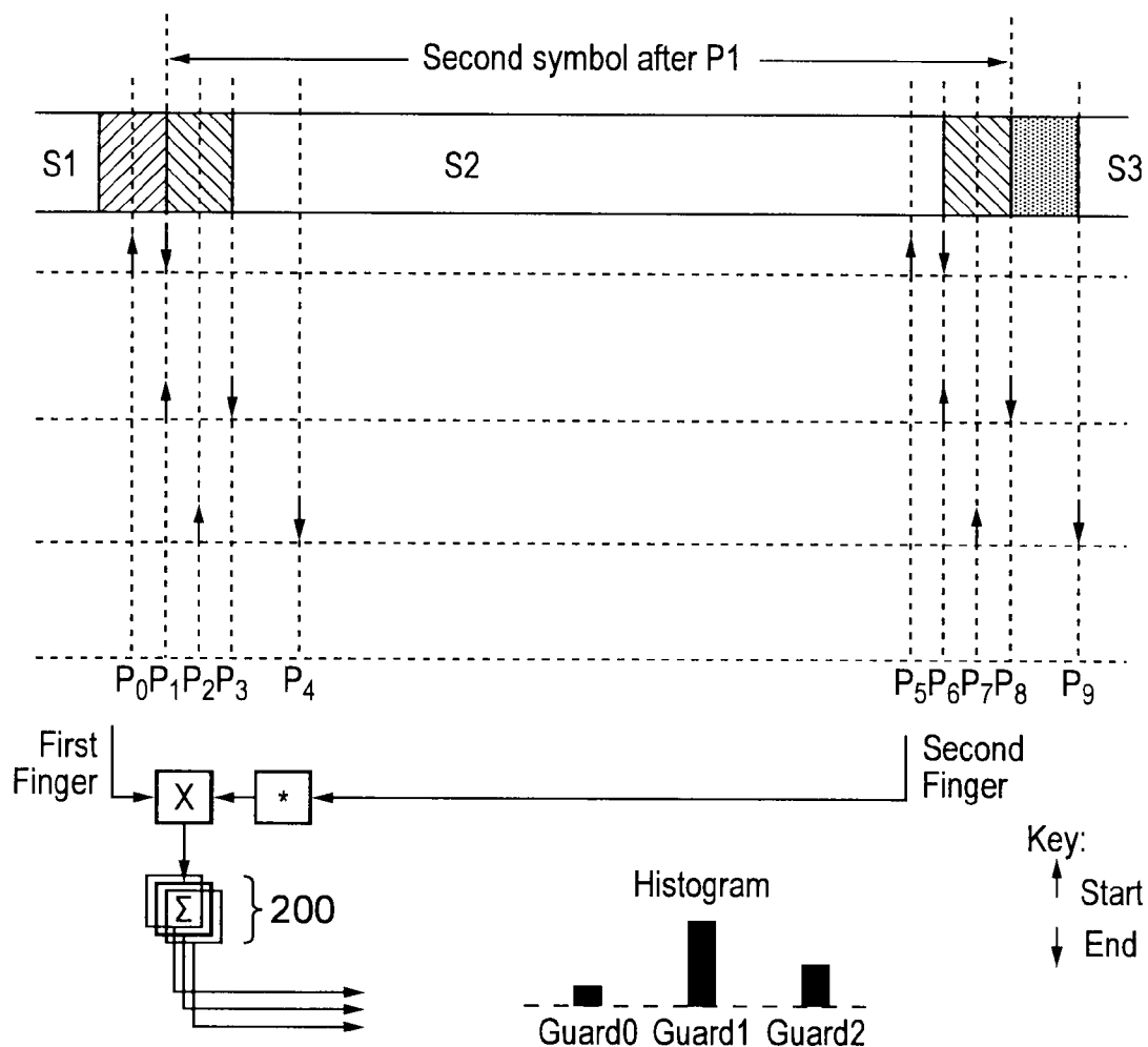
Operation of Simplified Architecture at Second Symbol
