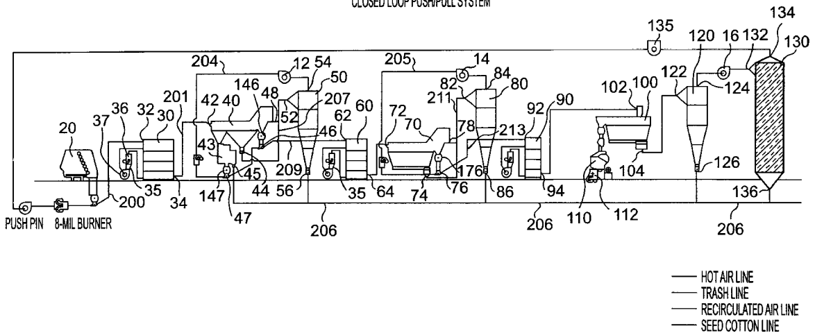
CLOSED LOOP PUSH/PULL SYSTEM
