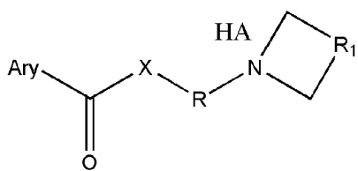
Structure 2c
