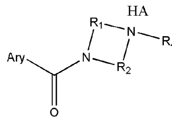
Structure 2d
