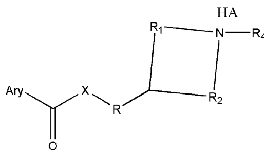
Structure 2b
