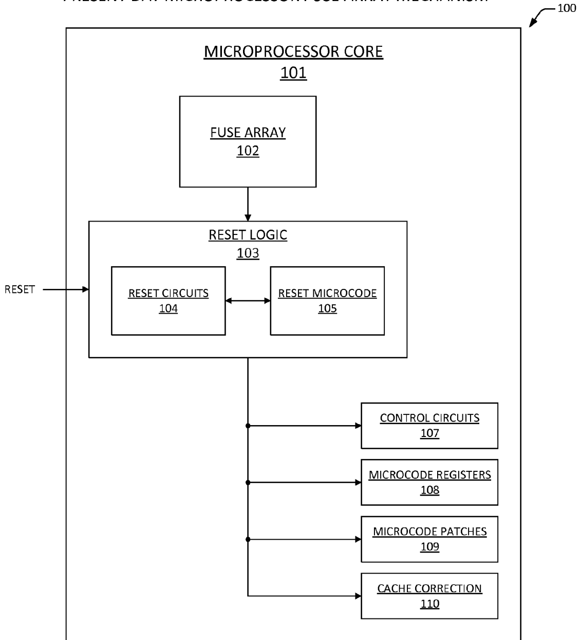
PRESENT DAY MICROPROCESSOR FUSE ARRAY MECHANISM
