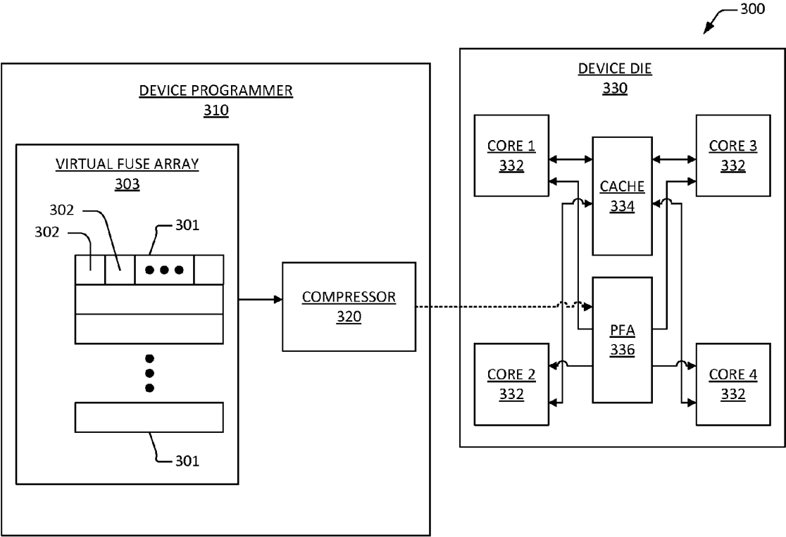
MICROPROCESSOR FUSE ARRAY COMPRESSION SYSTEM
