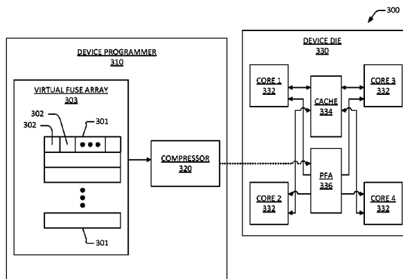
MICROPROCESSOR FUSE ARRAY COMPRESSION SYSTEM
