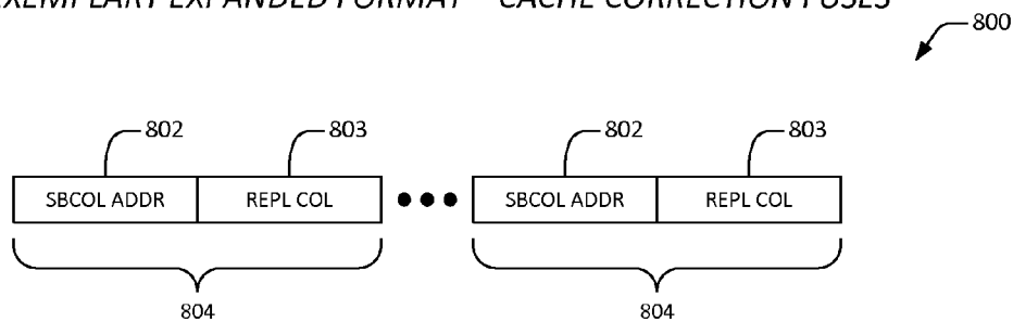
EXEMPLARY EXPANDED FORMAT – CACHE CORRECTION FUSES
