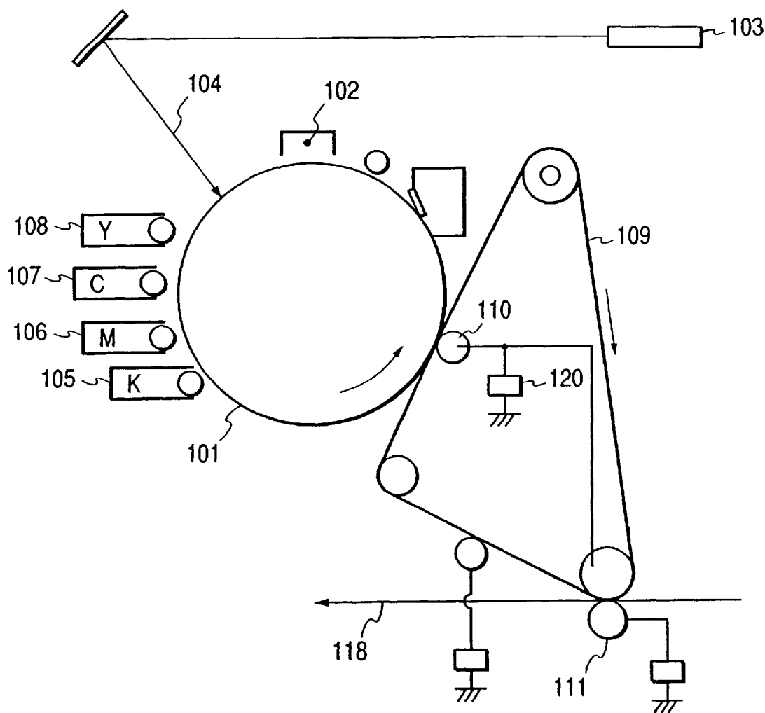
FIG. 5 PRIOR ART
